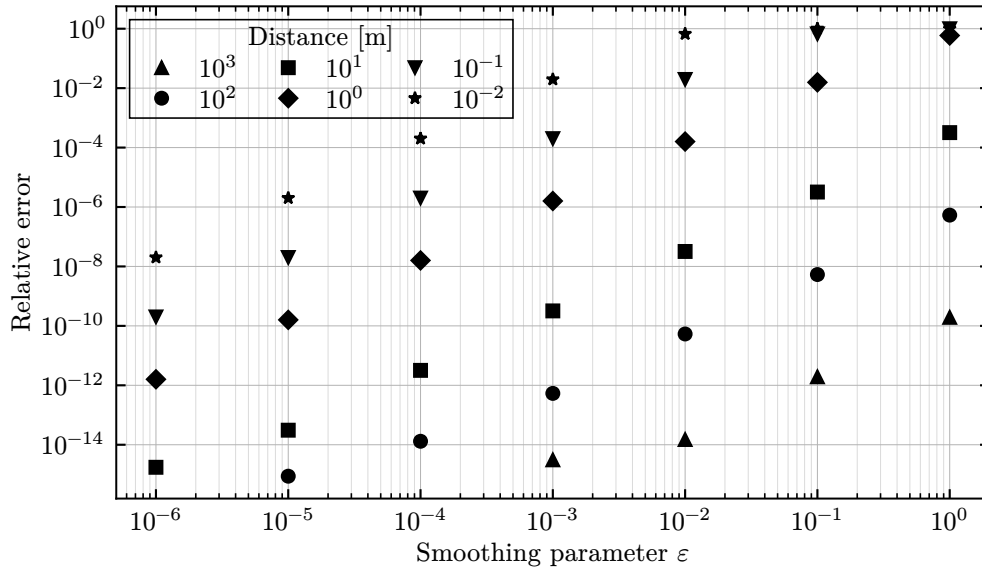
Figure 7: The relative error in induced velocity for different smoothing parameters, evaluated at varying distances from some vortex filament in a wind turbine wake.
