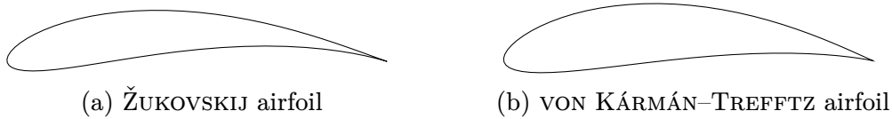
Figure 4: Two airfoils described respectively by equations (3.2) and (3.9), whose parameters are c = 1.4 and s = 1/4(i - 3/5) . The (?) is k = 1.94 .
