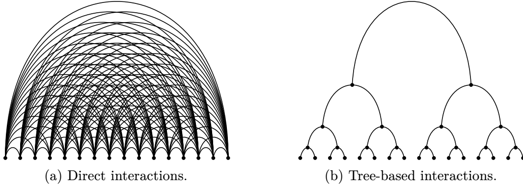
Figure 7: The difference in number of interactions for the direct and tree-based approaches.
