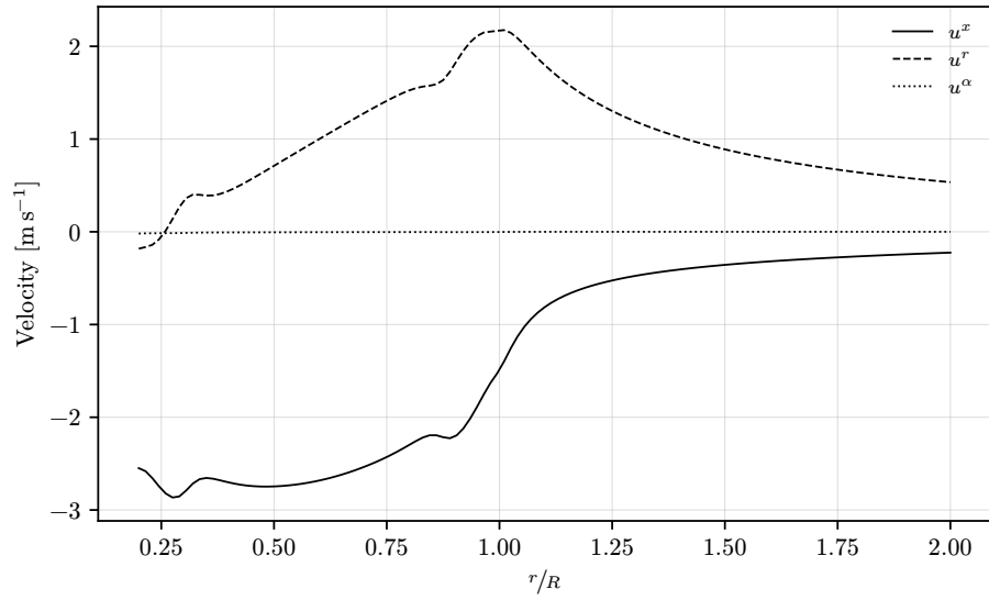
Figure 16: The average over the azimuth of all three cylindrical velocity components.
