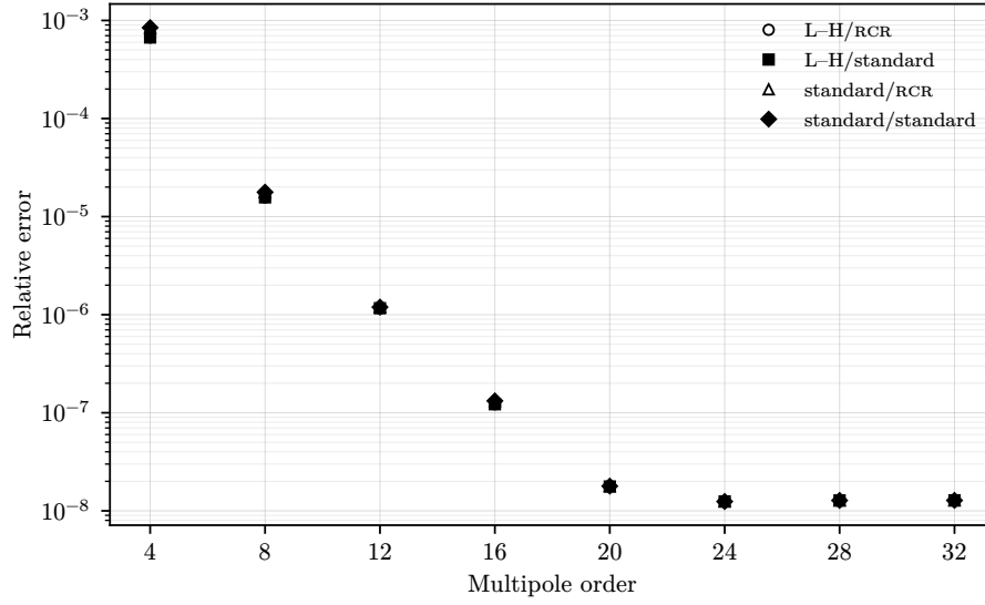
Figure 13: The relative error of the multipole induced velocity to the direct calculation at x = 1D .
