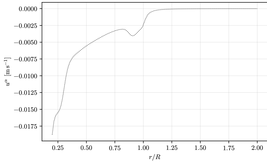
Figure 17: The average over the azimuth of the azimuthal velocity component.
