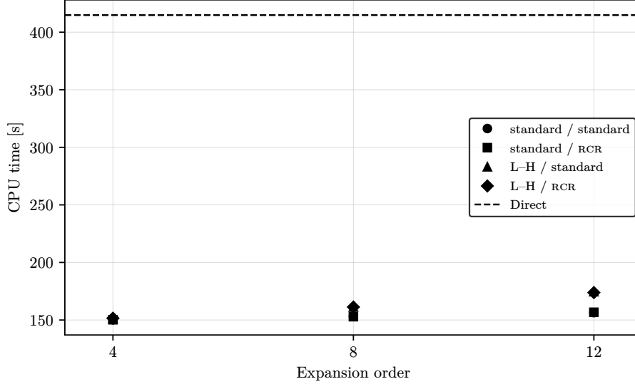
Figure 18: Median times of three benchmark CPU time measurements, comparing all fast multipole methods to the direct calculation.
