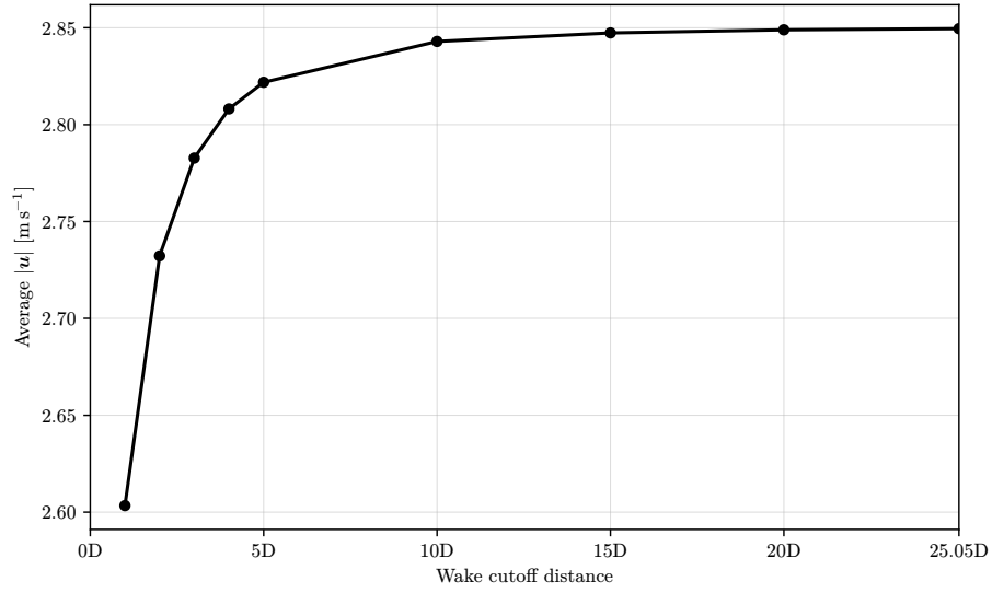
Figure 15: The weighted average of the velocity in the rotorplane calculated at different cutoff distances.
