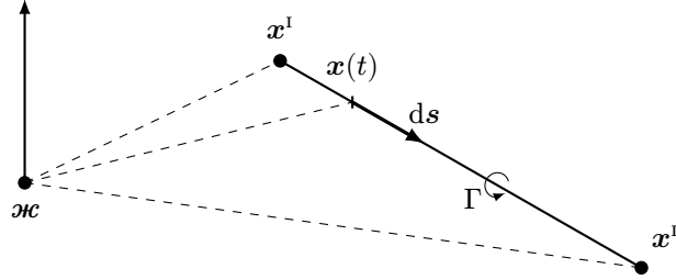
Figure 5: The calculation of the induced velocity from the vortex filament parametrized by \mathbf{x}(s) .
