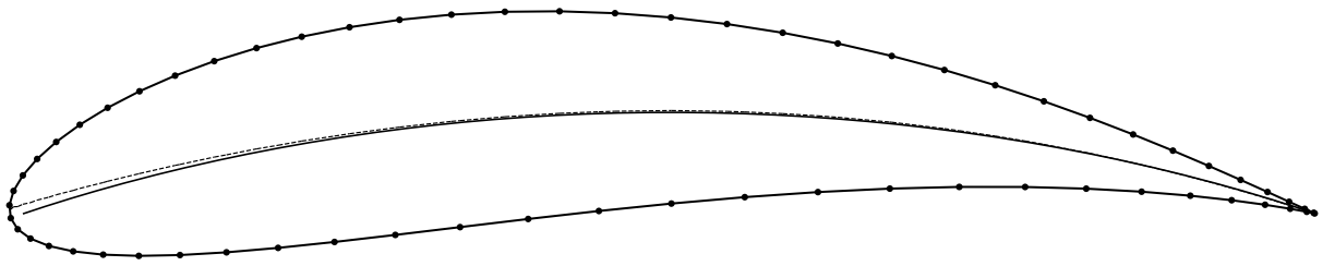
Figure 11: Mean camber line with skeleton of the VON KÁRMÁN-TREFFTZ airfoil
