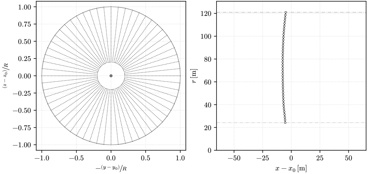
Figure 9: Every third evaluation point plotted. Number of r is 121. Number of \alpha is 180.
