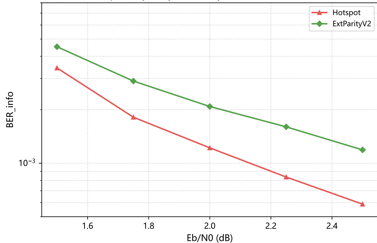
HotspotOnlyParity与ExtParityV2性能对比 (R≈0.348)
