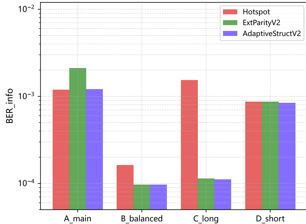
AdaptiveStructV2核心对比 ( R \approx 0.348 , E_b/N_0 = 2.0 dB)
