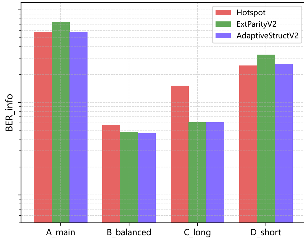
AdaptiveStructV2核心对比 ( R = 0.400 , E_b/N_0 = 2.0 dB)
