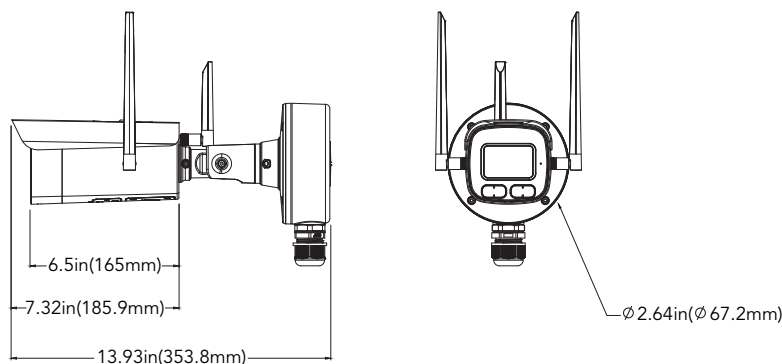
Camera Dimension
