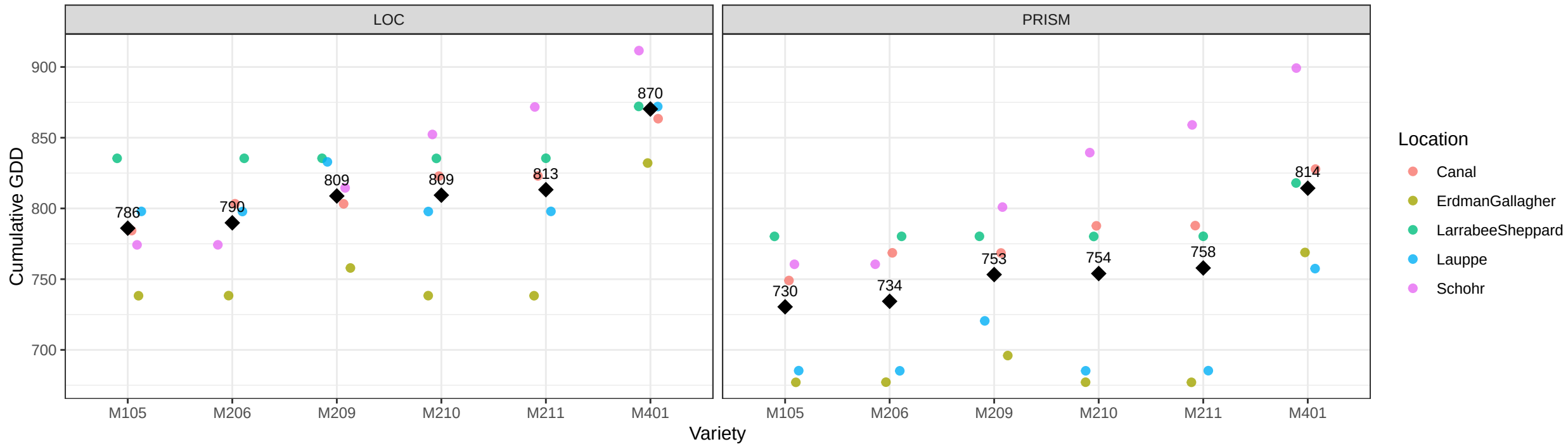
Cumulative GDD at PI by Variety
