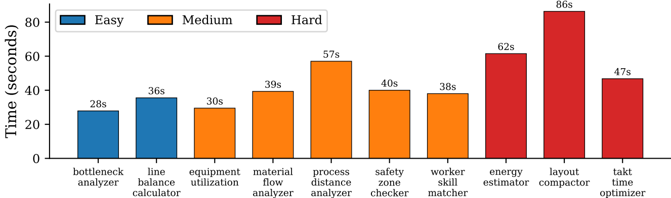
Adapter Generation Time by Tool
