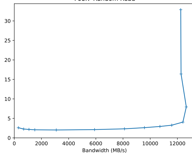
768K Random Read
