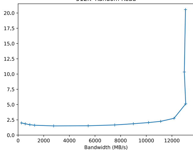
512K Random Read
