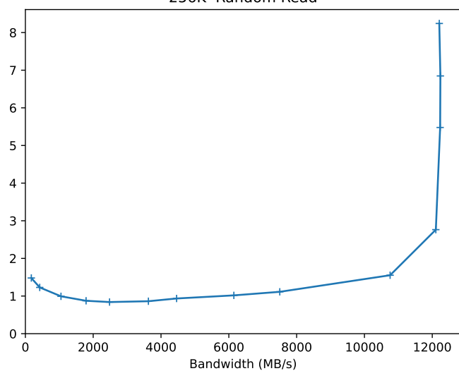
256K Random Read
