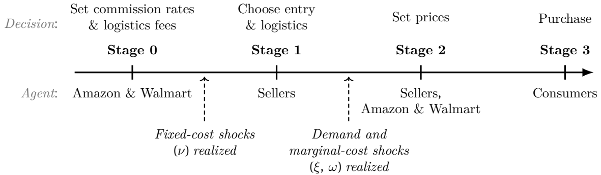
Figure 5: Model Timeline
