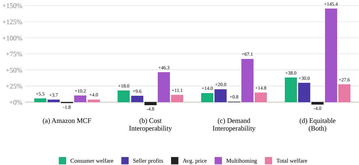
Figure A13: Interoperable Logistics Counterfactuals
