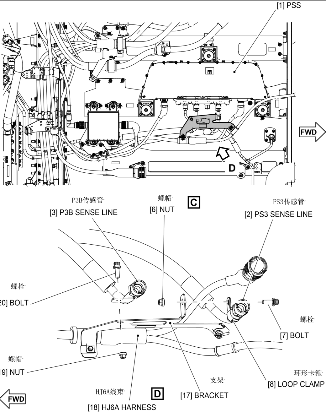
ICN-C919-A-732145-B-58828-07012-A-001-01 (2/2) PSS , PS3 sense line, and P3B sense line 图1 PSS、PS3传感管和P3B传感管(共2张第2张) ON A/C MSN ALL
