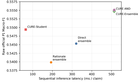
Figure 2: Descriptive compute-quality context. Macro-F1 is the reported raw-official P1 point estimate; latency is sequential inference measured on a common 256-claim validation subset. The axes therefore summarize two frozen artifacts and do not constitute a paired effectiveness-cost test.
