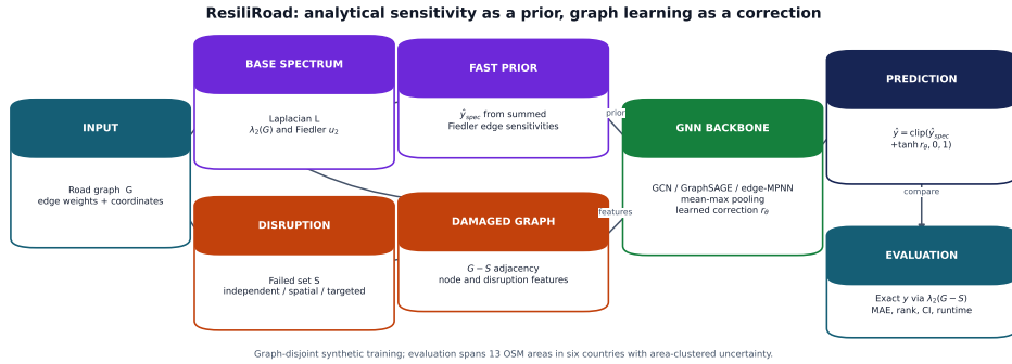
Figure 1: ResiliRoad workflow. Exact damaged-graph eigendecomposition constructs labels only. The intact Fiedler vector produces both an optional node feature and the explicit first-order prior; the selected GNN backbone learns a bounded correction.
