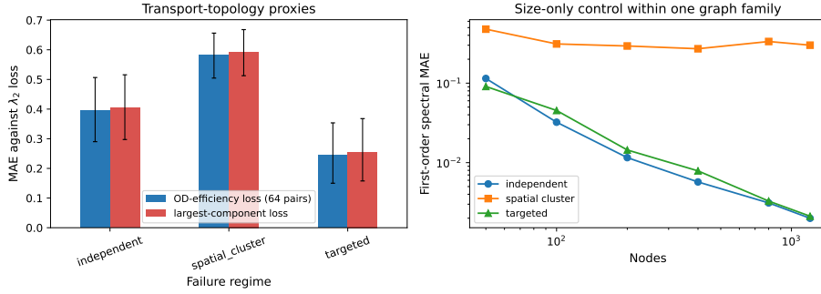
Figure 7: Reviewer-motivated controls. (a) Topology-only transport-proxy error against the algebraic-connectivity-loss target. (b) First-order spectral error as graph size changes within one planar road-like graph family.
