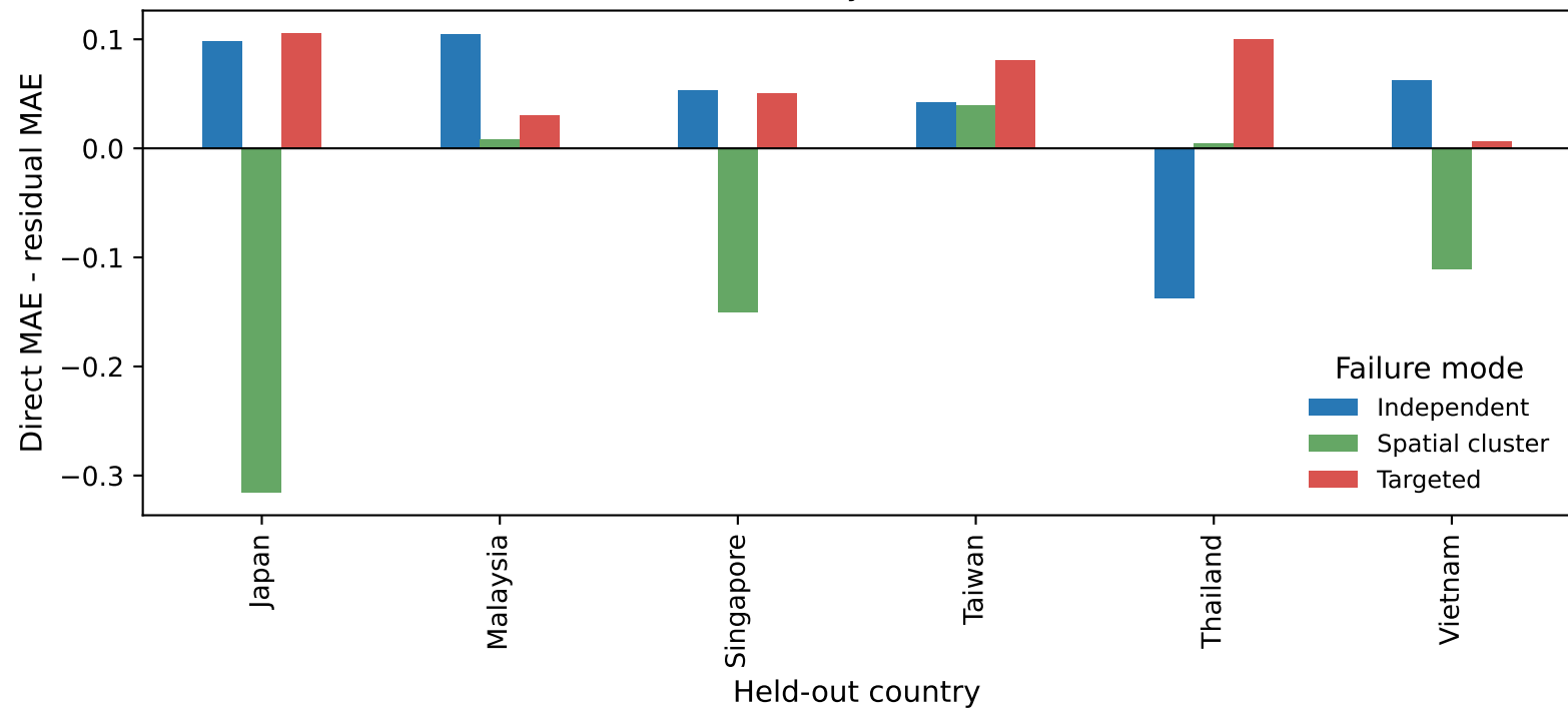
Leave-one-country-out OSM transfer
