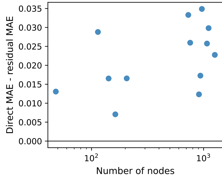
Spearman \rho=0.40
