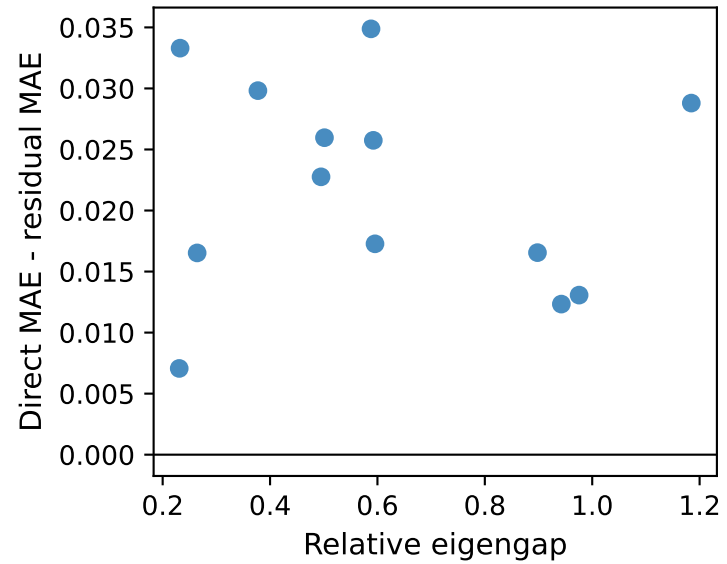
Spearman \rho=-0.11
