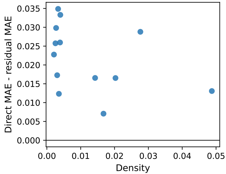
Spearman \rho=-0.35
