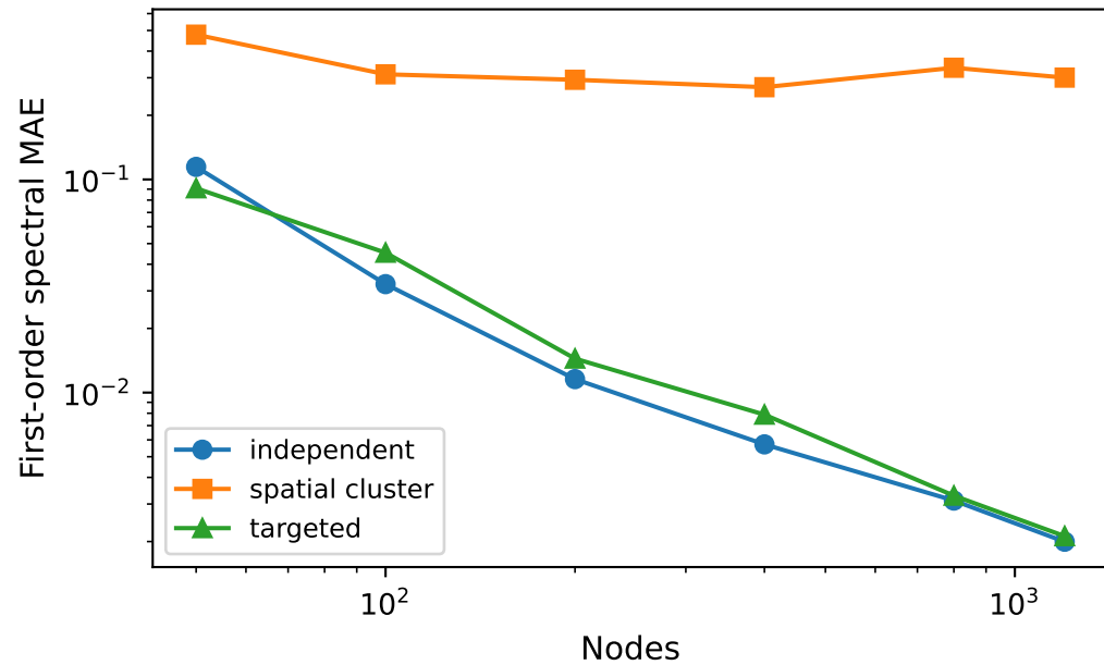
Size-only control within one graph family
