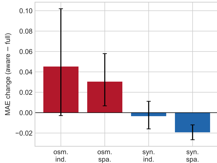
(c) Reliability-context ablation
