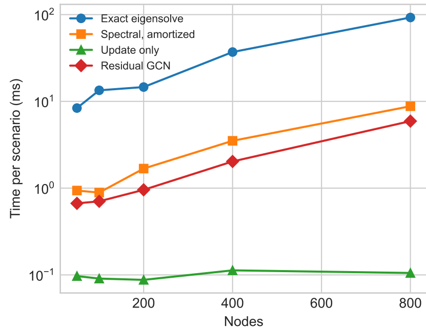
(a) Controlled scaling
