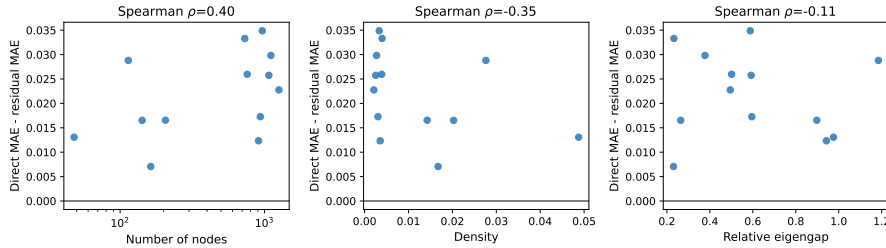
Figure 5: Descriptive residual-GCN gain versus OSM graph size, density, and relative eigengap. Each point is one area averaged over seeds and failure regimes; positive values favour residual prediction.
