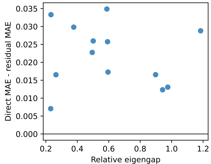
Spearman \rho=-0.11
