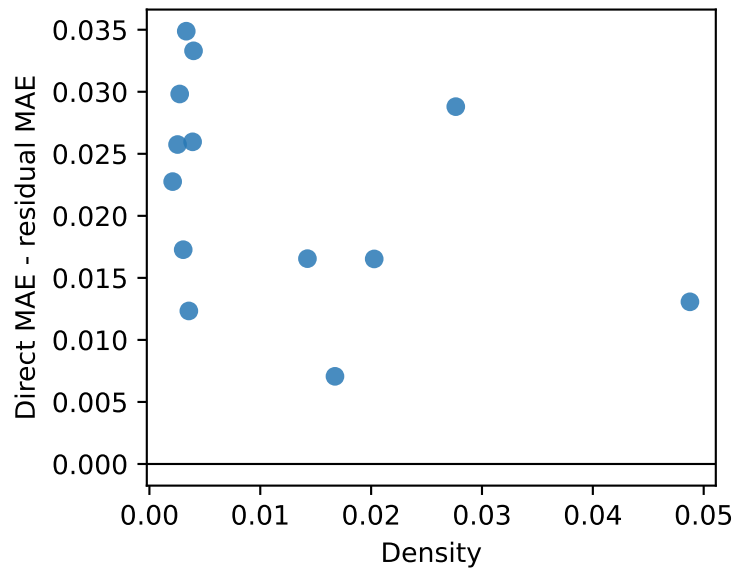
Spearman \rho=-0.35
