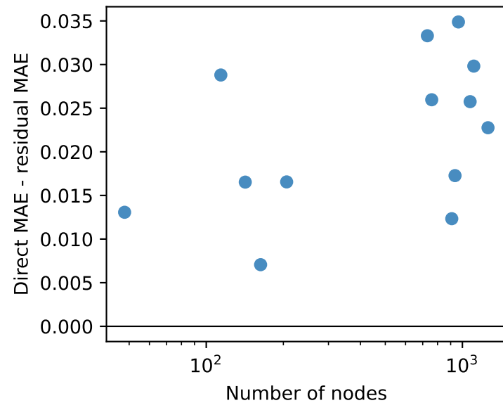
Spearman \rho=0.40
