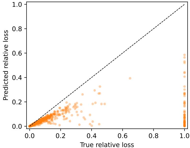
Spectral first order
