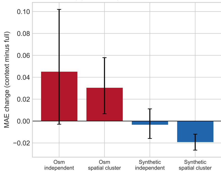
(b) Reliability-context ablation
