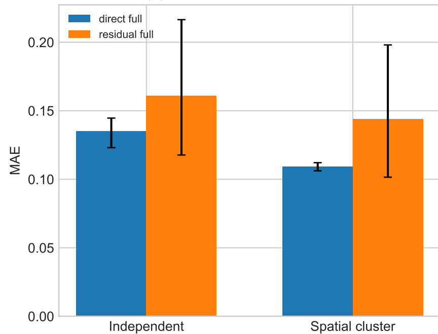
(a) Leave-one-area-out OSM
