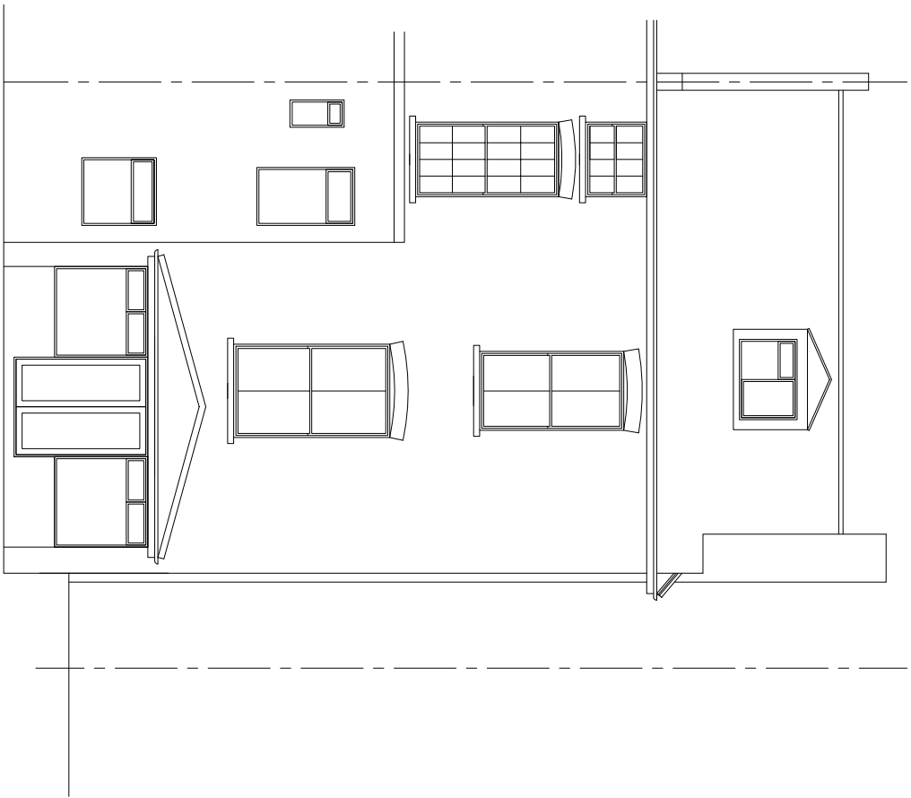
REAR ELEVATION
