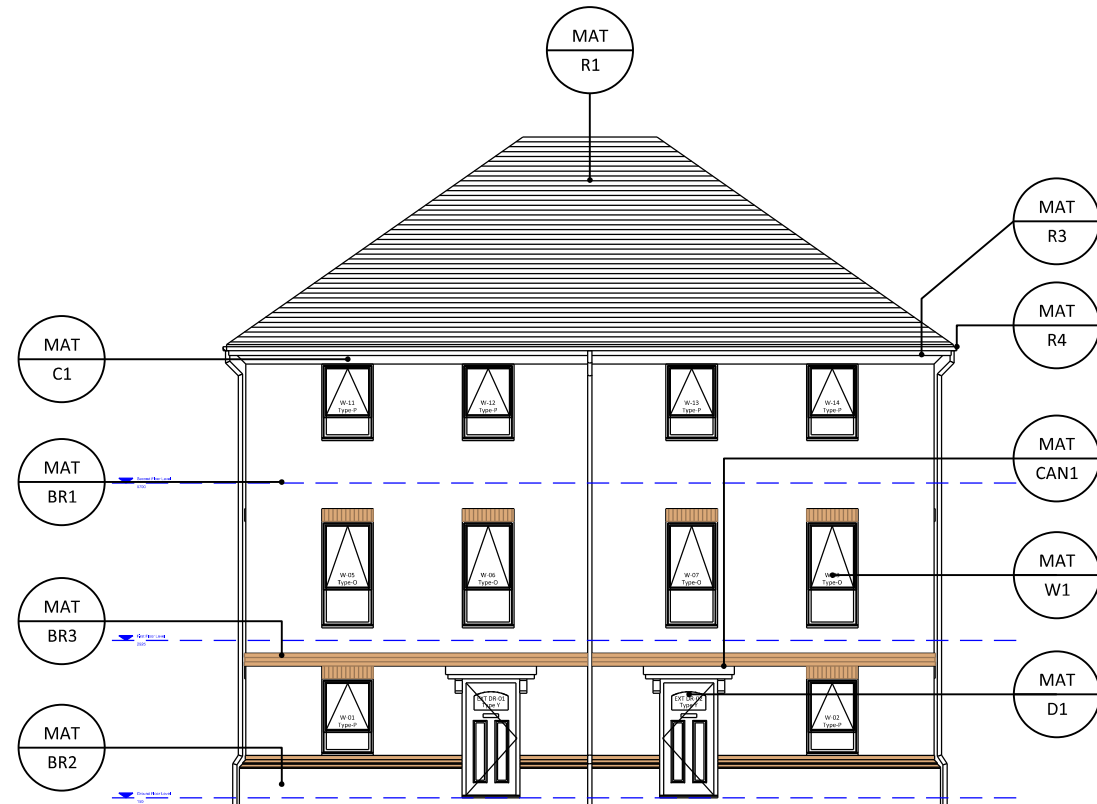
KEY ELEVATION(S) - HOUSES PLOTS 81-81, 85-86, 89-90
