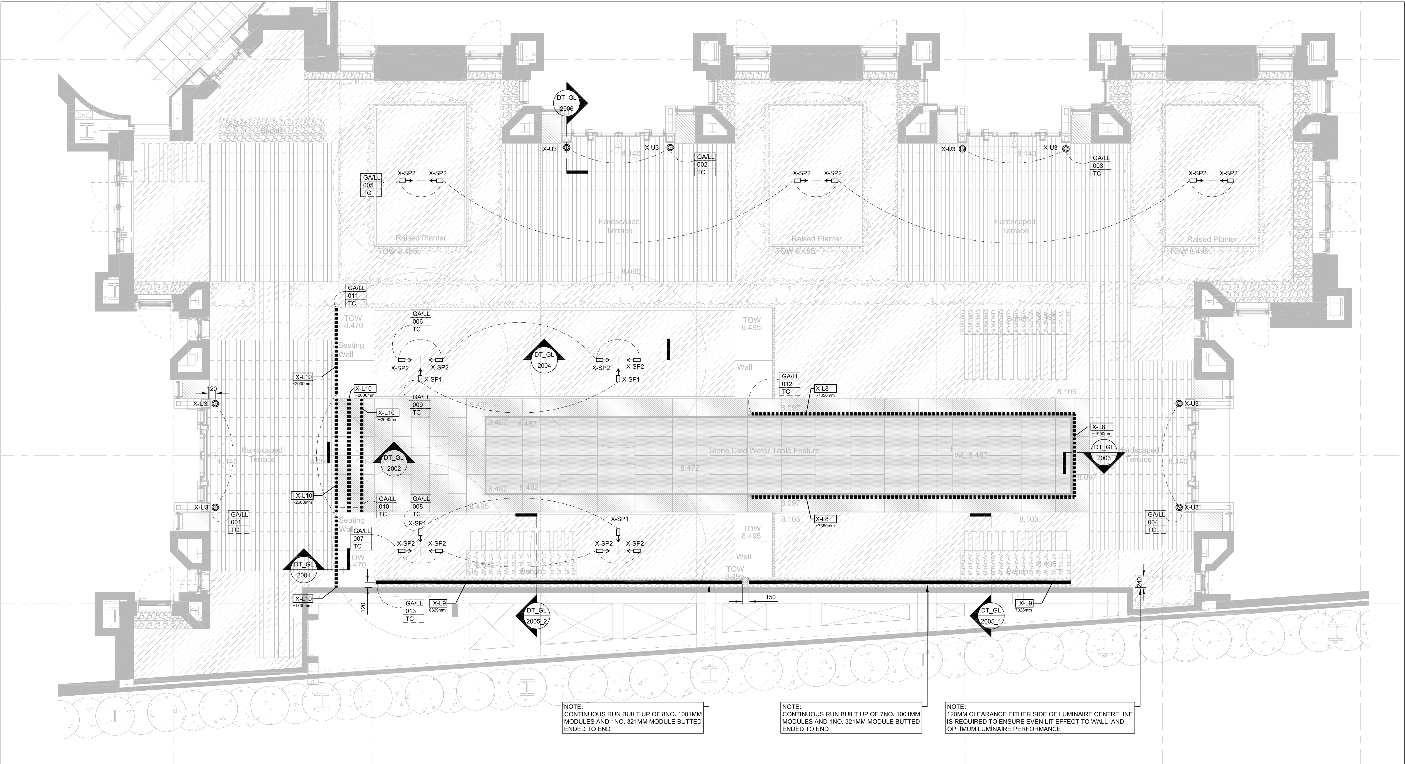
1 - GARDEN LEVEL - GA - SCALE 1:50
