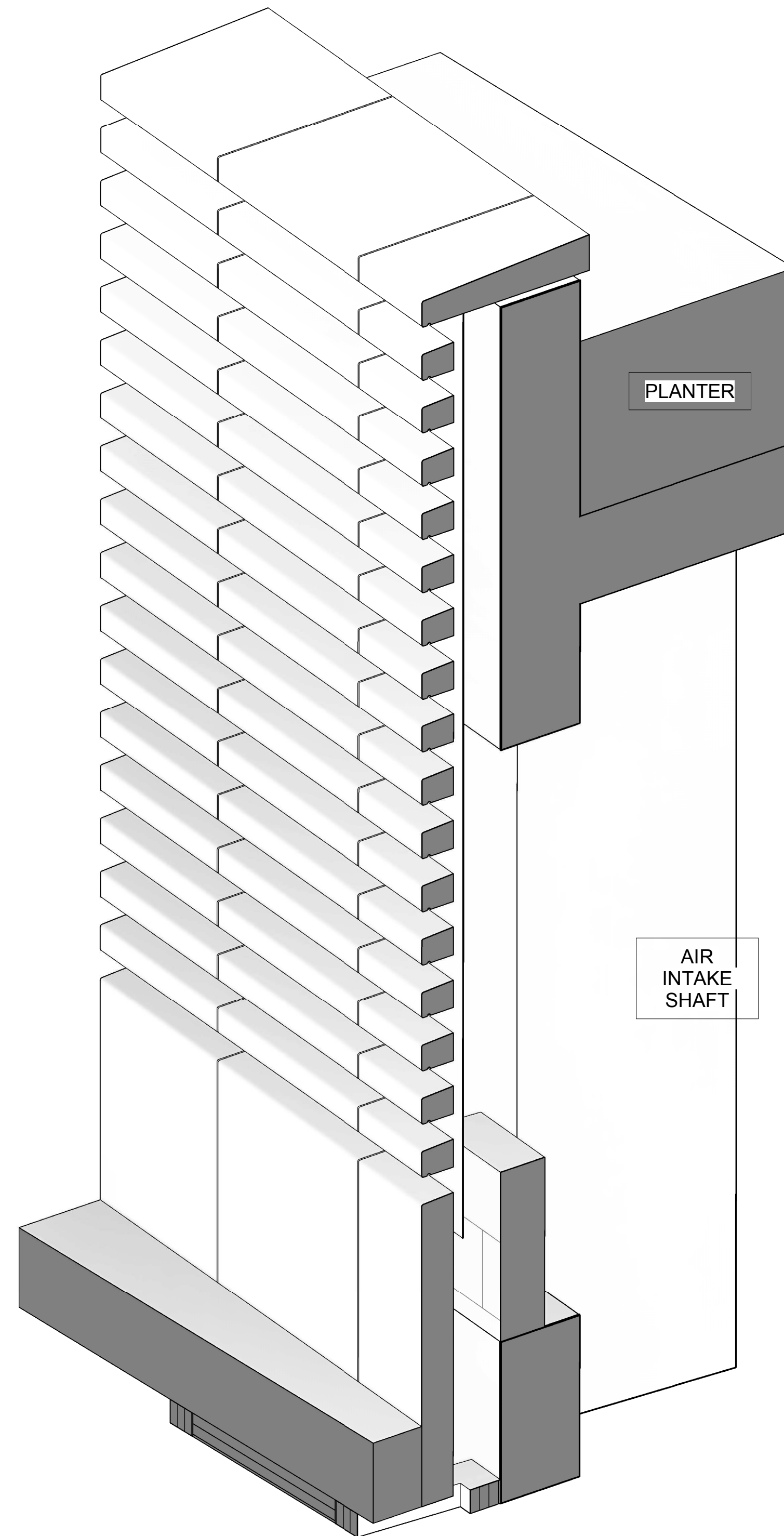
4 580-21 - Garden Airwell Axo
