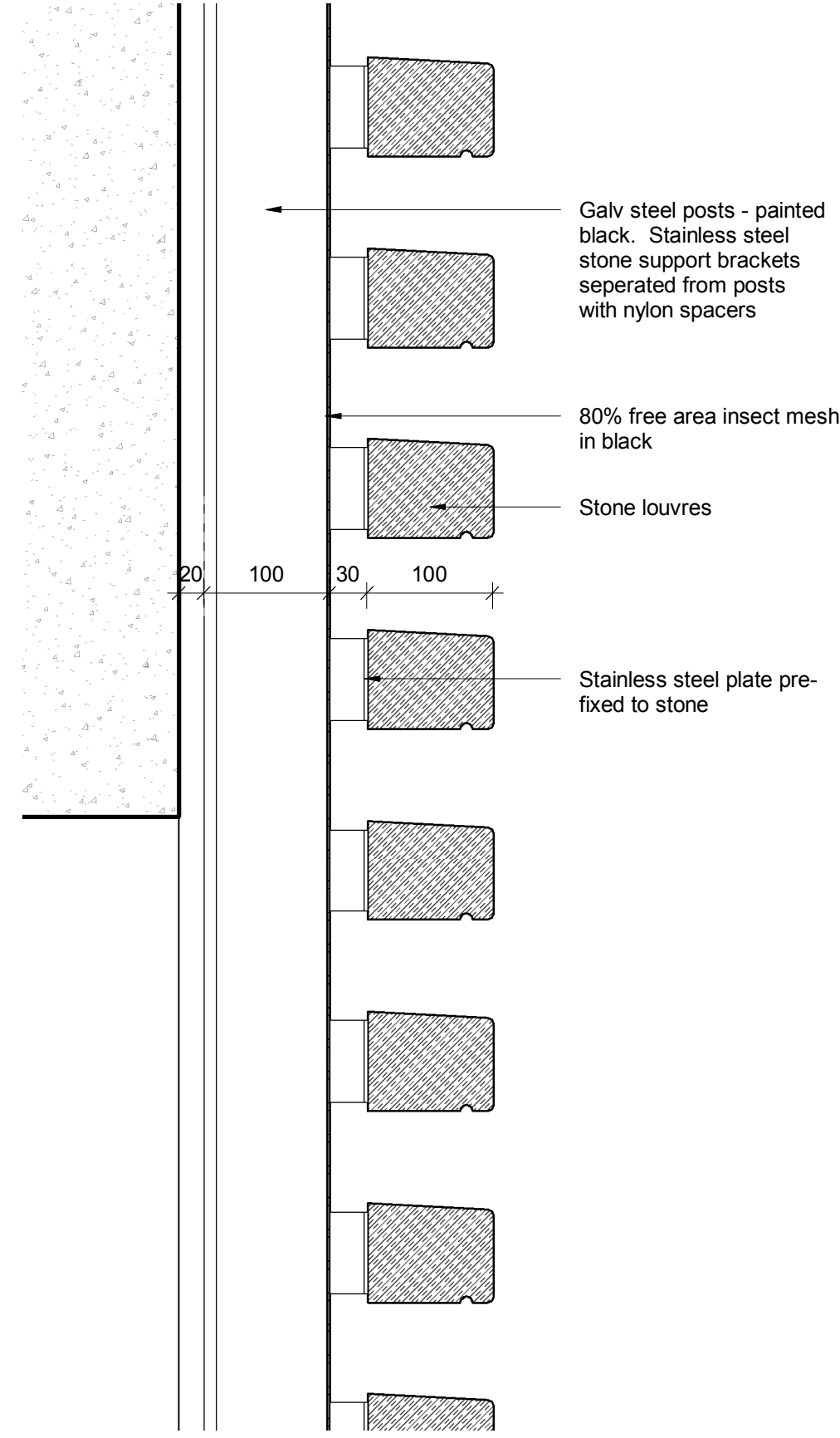
3 580-23 - Section 1:5
