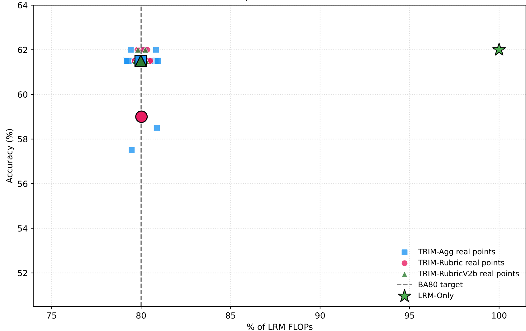
OmniMath Mixed 3-4/4-9: Real Dense Points Near BA80
