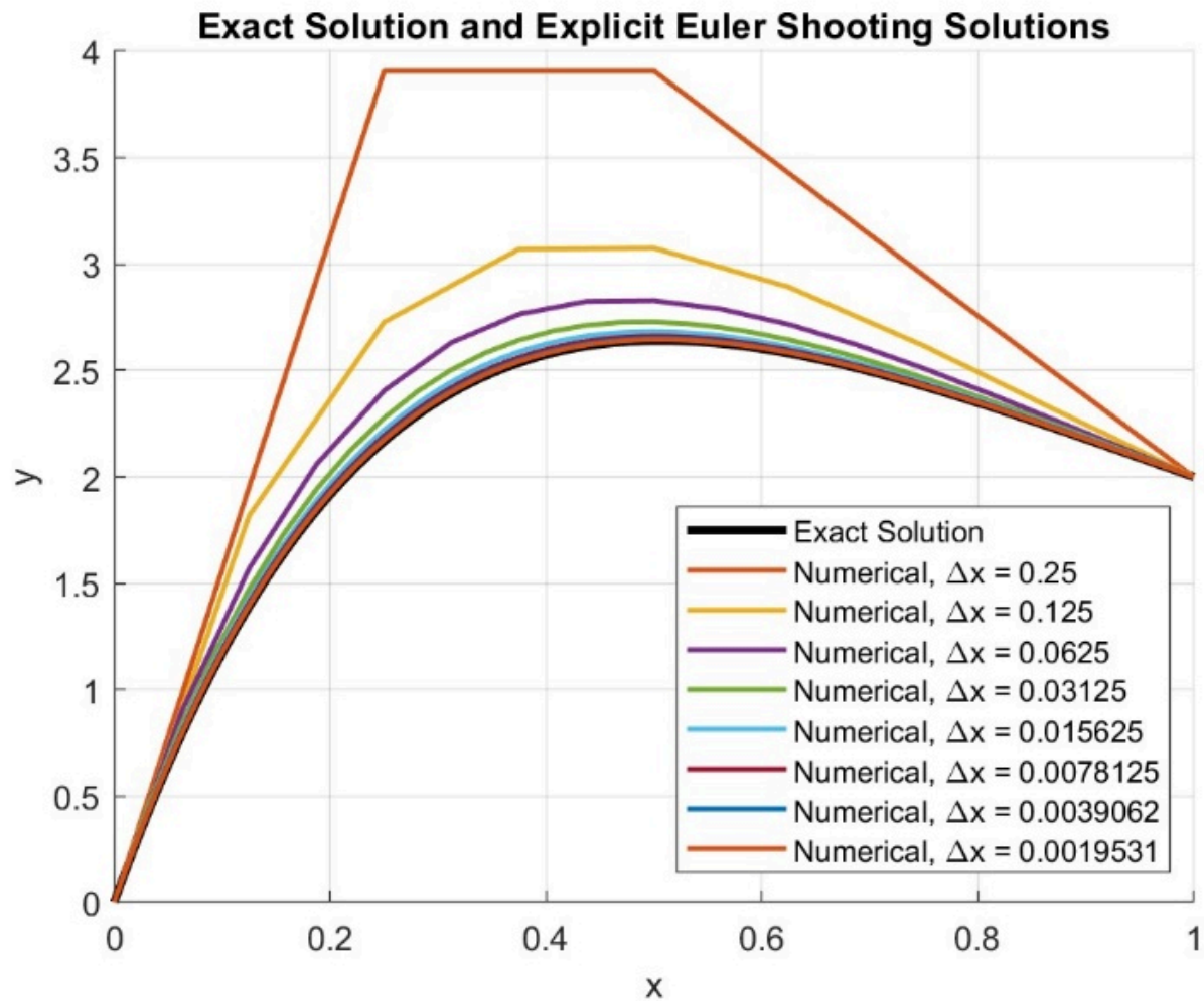
Figure 9. Comparison of analytical solutions and numerical solutions under different conditions (Explicit Euler Method)
