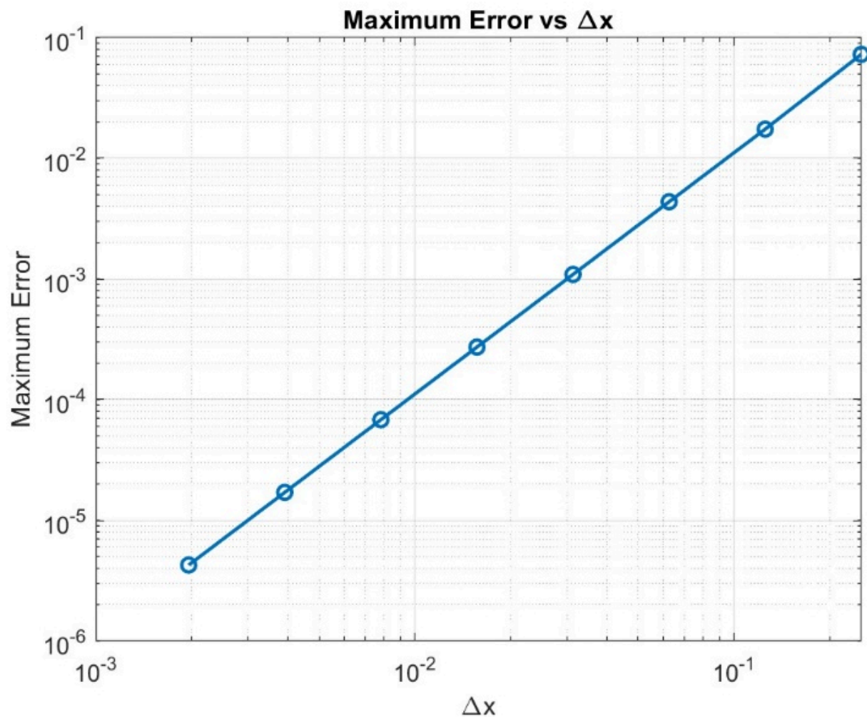
Figure 11. Maximum Error and relationship diagram (Crank-Nicolson Method)
