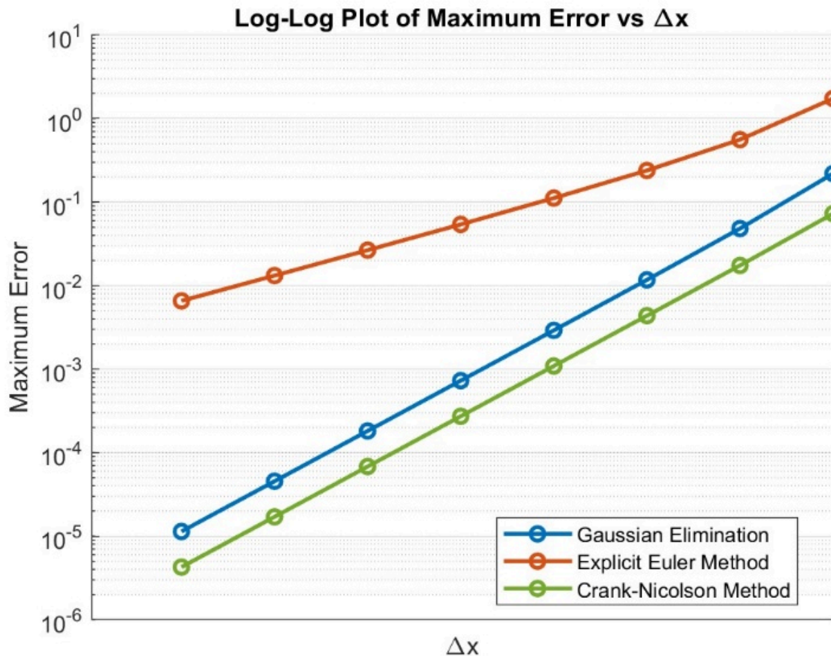
Figure 13. Maximum Error and relationship diagram (comparison of three methods)
