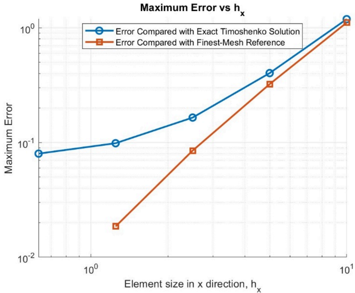
Figure 18. Relationship between maximum error and element side length
