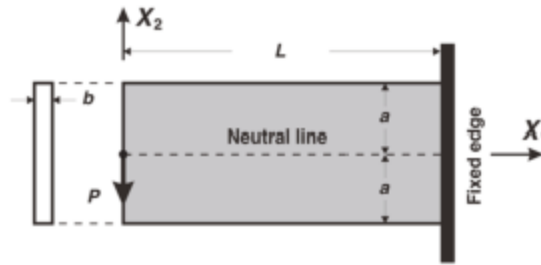
Figure 1: Schematics of the cantilever beam.
