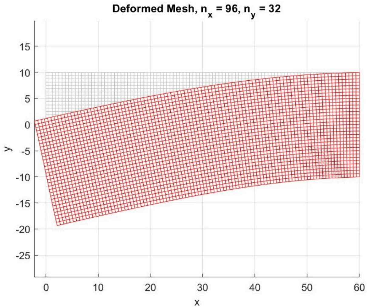
Figure 20. The xy position diagram of the densest grid when it is stressed
