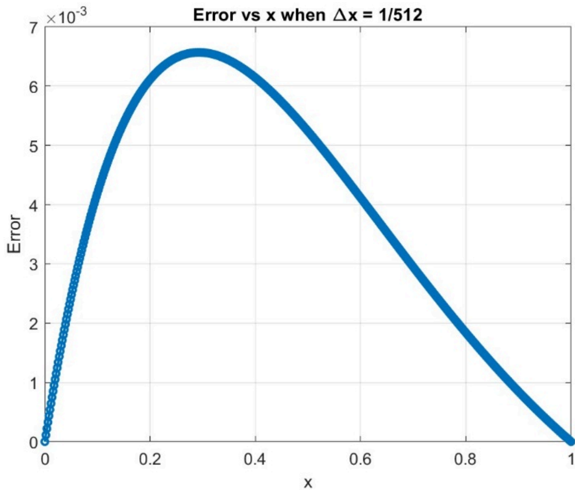
Figure 10. Error absolute value distribution at that time (Explicit Euler Method)
