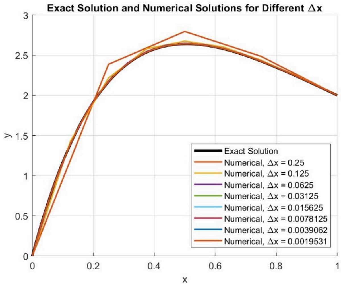
Figure 2. Comparison of analytical solutions and numerical solutions under different conditions (Gaussian Elimination)
