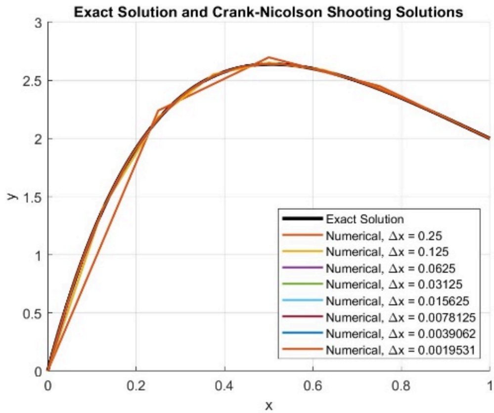
Figure 14/Figure 15/Figure 16, comparison chart of analytical solution and numerical solution under different conditions (comparison of three methods)
