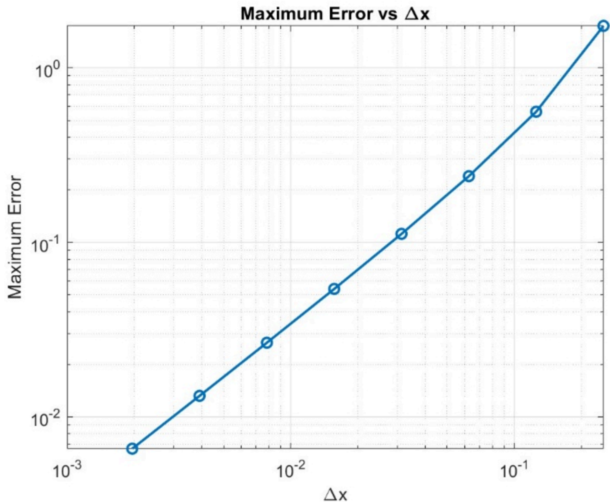
Figure 8. Maximum Error and relationship diagram (Explicit Euler Method)
