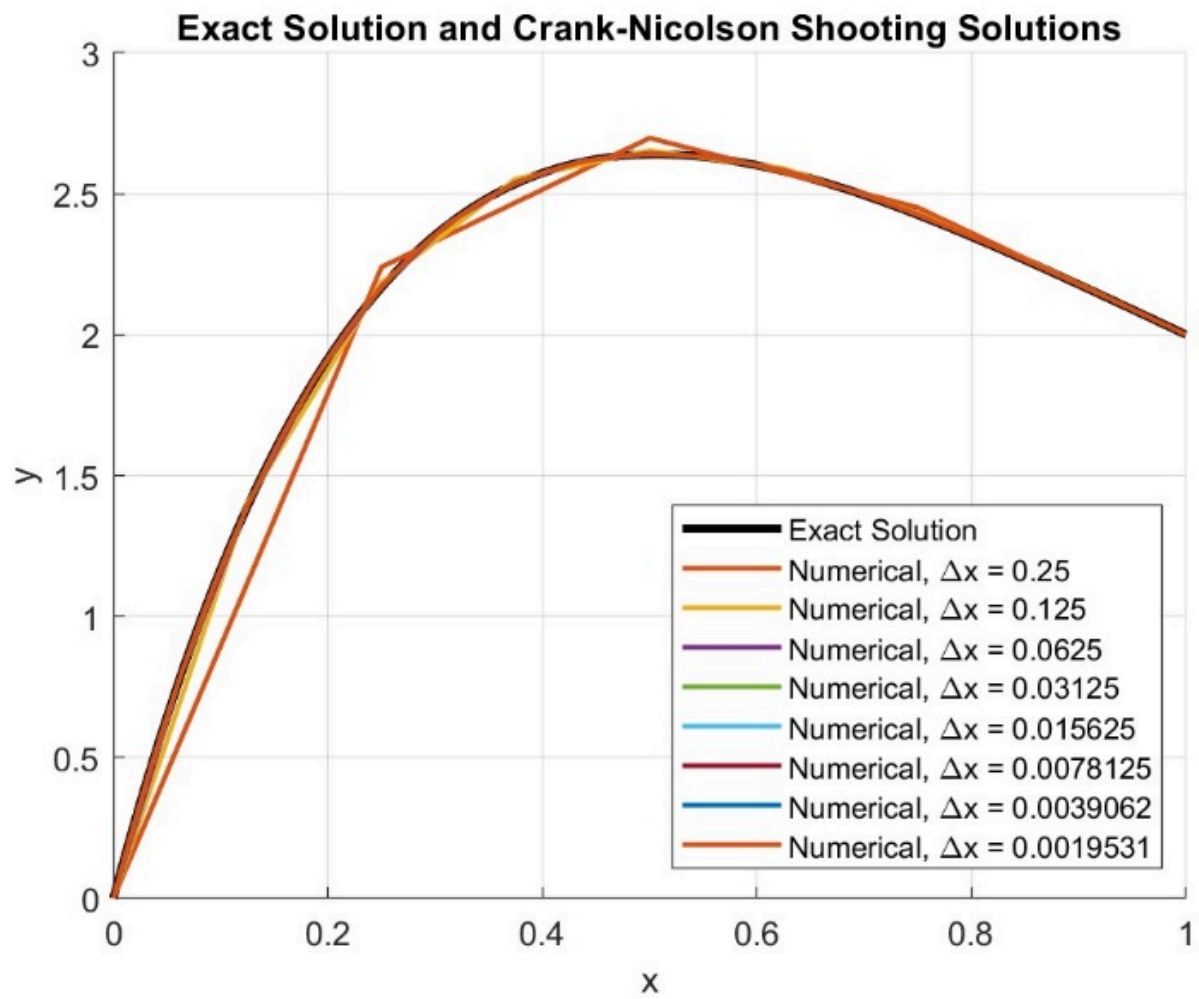
Figure 12. Comparison of analytical solutions and numerical solutions under different conditions (Crank-Nicolson Method)
