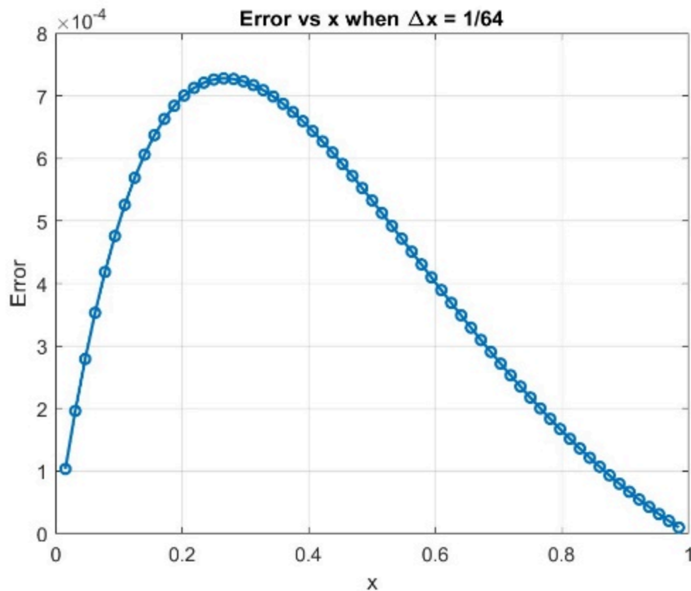
Figure 4/Figure 5/Figure 6/Figure 7. Error absolute value distribution (Gaussian Elimination) at different times
