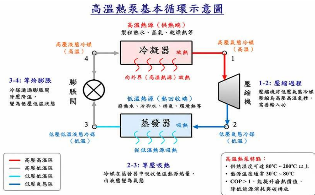
Figure 5, basic cycle diagram of high temperature heat pump
