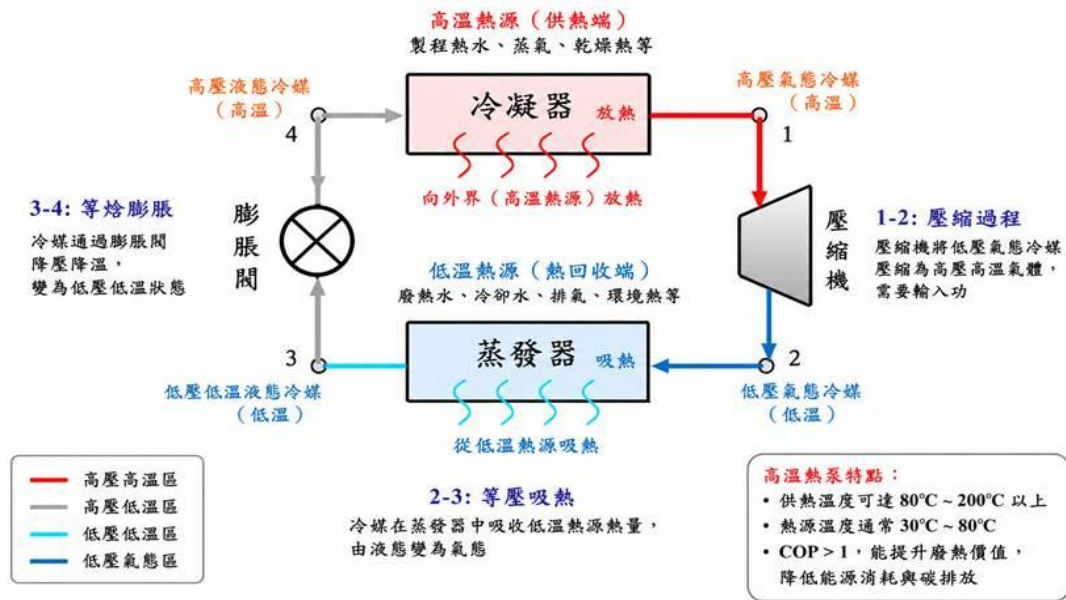
Figure U, basic cycle diagram of high temperature heat pump
