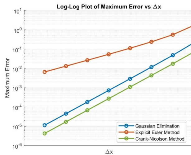
Figure 13. Maximum Error and relationship diagram (comparison of three methods) \Delta x
