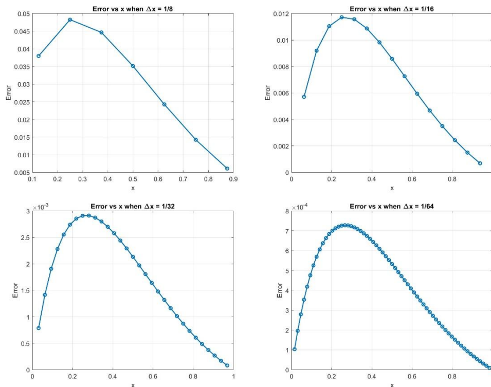
Figure 4/Figure 5/Figure 6/Figure 7. Error absolute value distribution (Gaussian Elimination) at different times Δx
