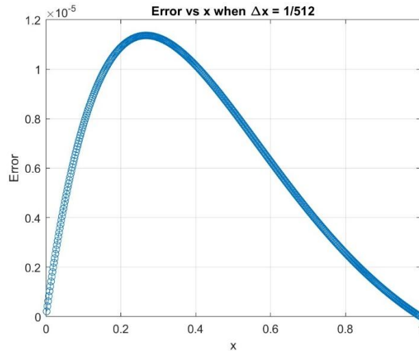
Figure 3. Error absolute value distribution (Gaussian Elimination) at that time \Delta x = 1/512
