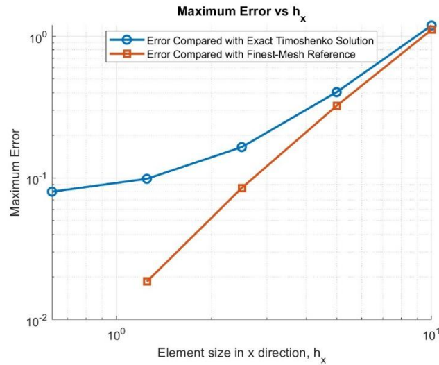
Figure 18. Relationship between maximum error and element side length h Table 8 calculates the error values under different grids. It can be found that when the grid is finer, the error between the numerical solution and the correct solution will be smaller. And it can be seen from Figure 17 that when the grid density increases, the relationship between the displacement and the position will be closer to the curve of the correct solution. When the grid is the
