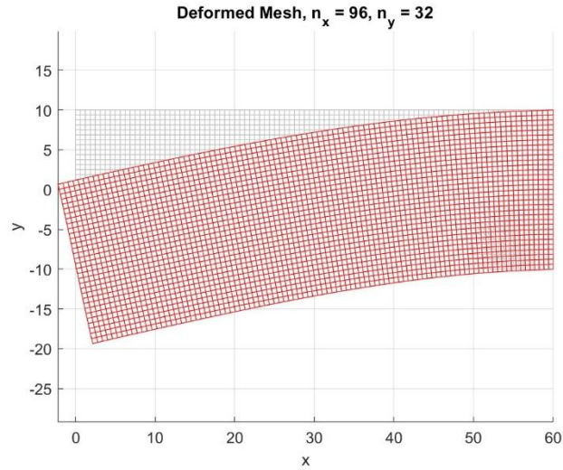
Figure 20. The xy position diagram of the densest grid when it is stressed Here we also express the stress and non-stress conditions when the grid is densest with the most intuitive xy position diagram. If we observe the position of , we can find that the vertical displacement of the center point is consistent
