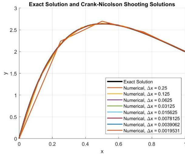
Figure 12. Comparison of analytical solutions and numerical solutions under different conditions (Crank-Nicolson Method) \Delta x
