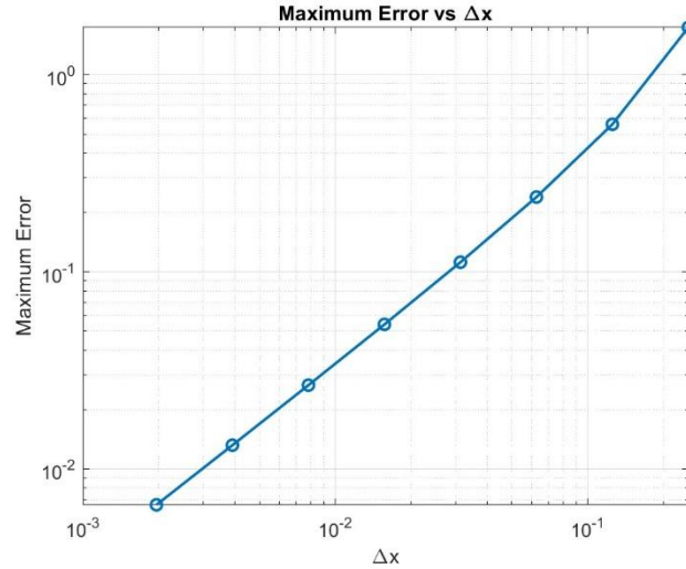
Figure 8. Maximum Error and relationship diagram (Explicit Euler Method) \Delta x
