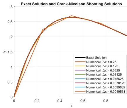
Figure 14/Figure 15/Figure 16, comparison chart of analytical solution and numerical solution under different conditions (comparison of three methods) \Delta x
