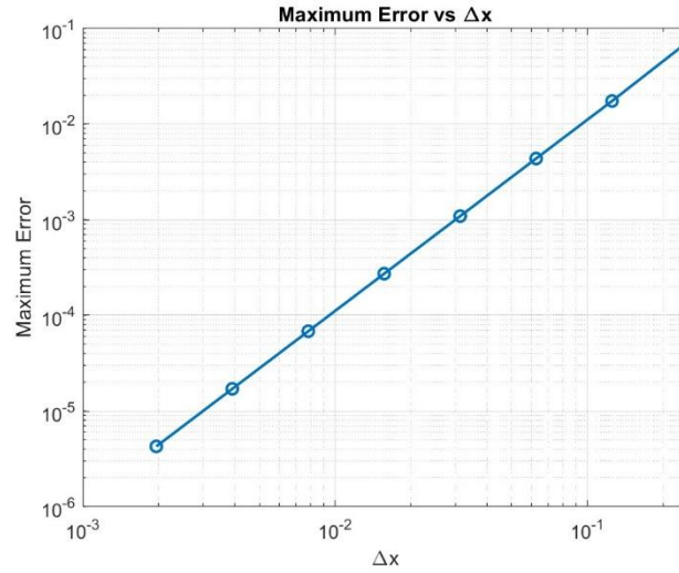
Figure 11. Maximum Error and relationship diagram (Crank-Nicolson Method) \Delta x
