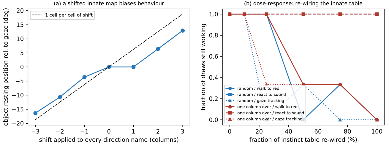
Supplementary Fig. 3 Blurred innate wiring (R7). (a) Resting position of the object relative to the gaze centre as a function of an imposed shift of every direction-bearing name in the table; (b) survival of three behaviours as a function of the fraction of the table that has been re-randomised or shifted by one column. Sources: 日志_整体偏移_正前方_新.log, 日志_存活曲线_新.log.
