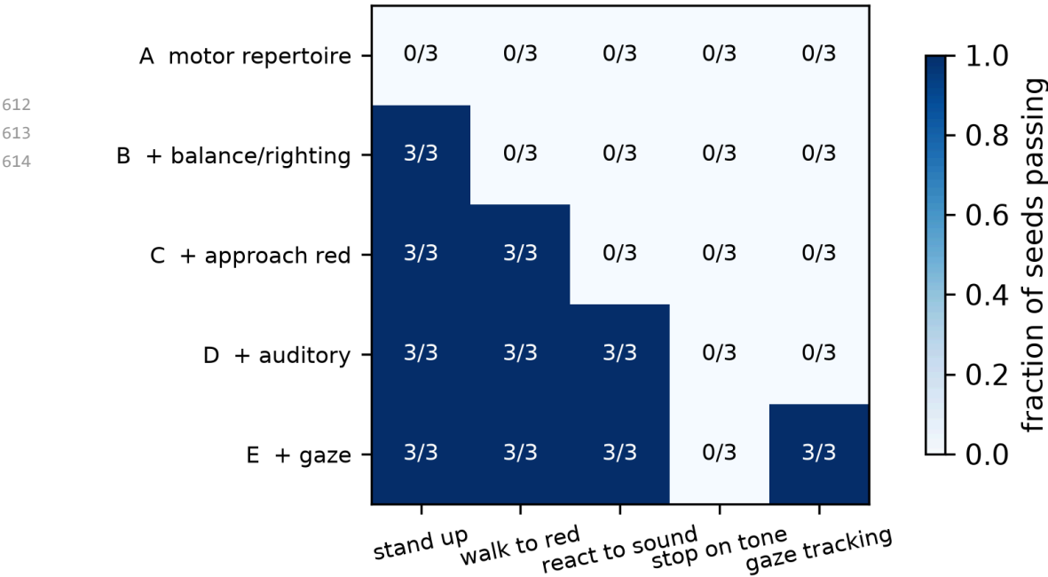
Figure 4 The repertoire grows as instinct groups are added (3 seeds per stage)
