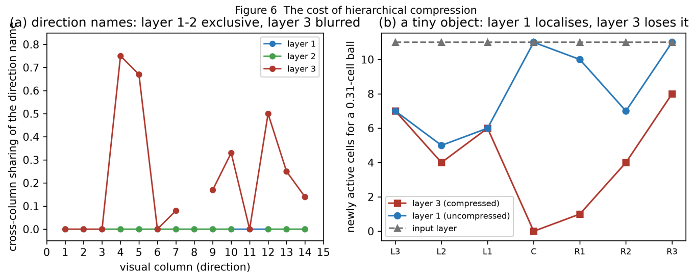
Supplementary Fig. 2 The cost of hierarchical compression (R5). (a) Cross-column sharing of direction names in layers 1, 2 and 3 of the visual hierarchy; (b) for a ball one third of a cell across, the columns in which each layer's newly active cells lie. Sources: 日志_方位分辨率.log, 日志_前几层.log.
