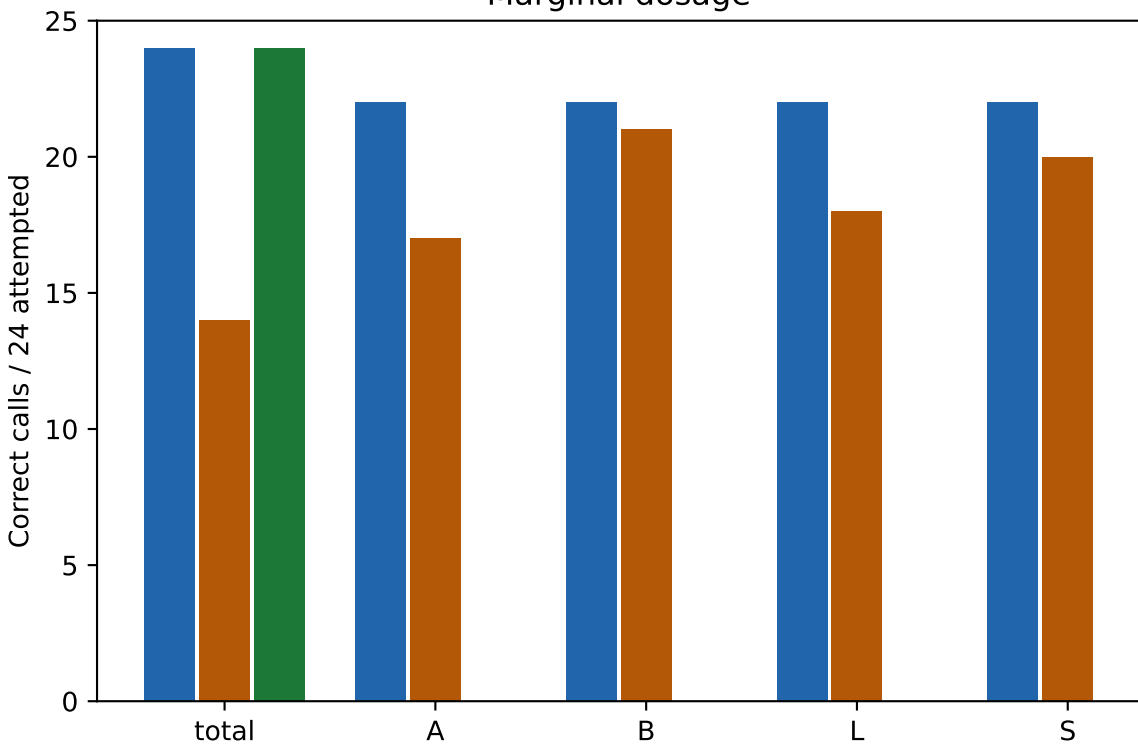
Held-out donors within the assembly panel; structural ranking is not physical phase Marginal dosage Structural-pair imputation
