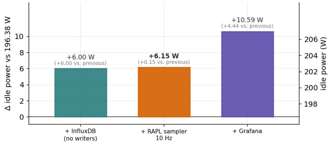
Figure 3. Overhead of Different Applications
