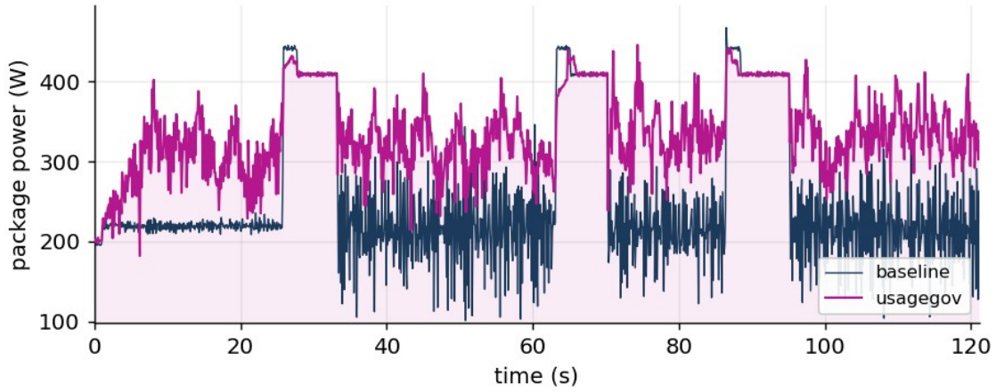
Figure 11. Governor (usagegov) in Action
