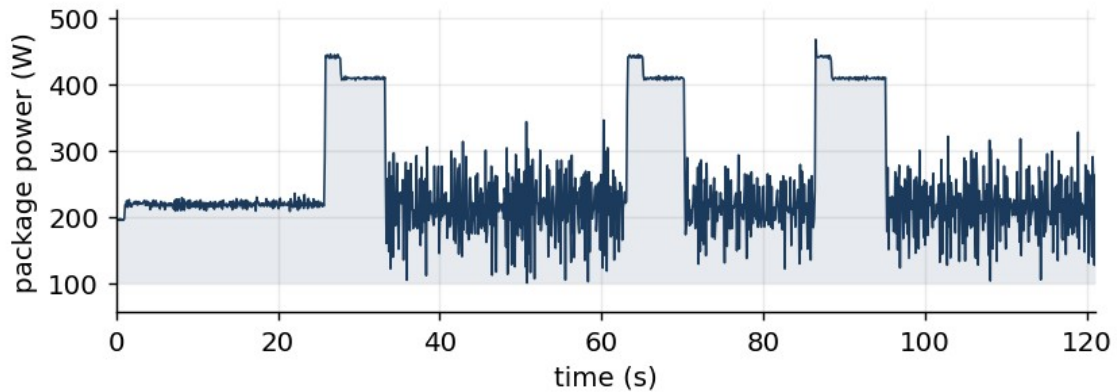
Figure 15. AI Sim 2 workload
