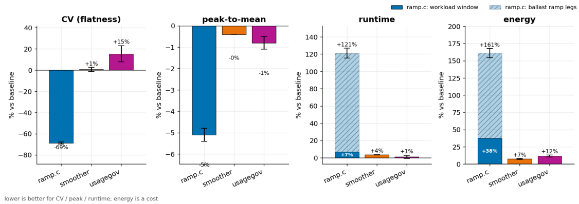
Figure 20. Grid Results for all Three Smoothers
