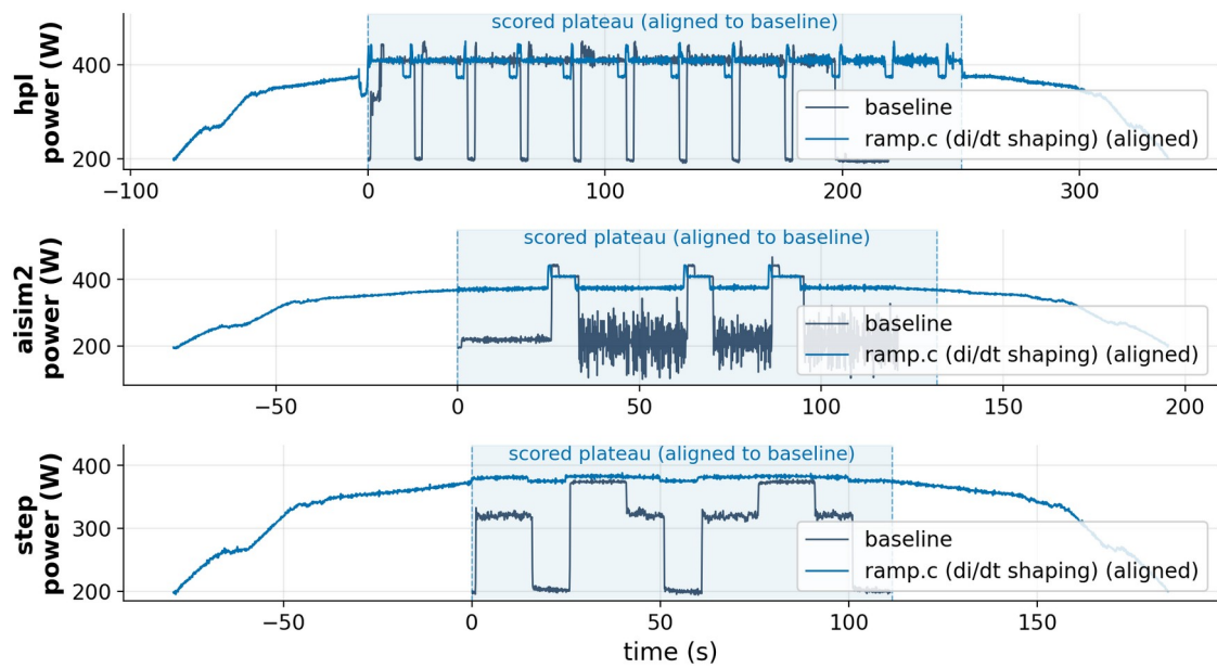
Figure 17. ramp.c vs workloads
