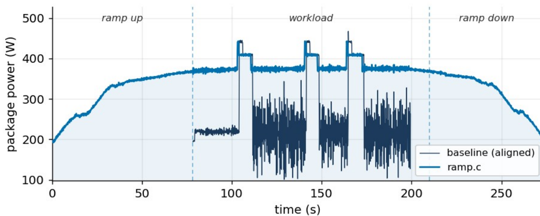
Figure 9. ramp.c in Action
