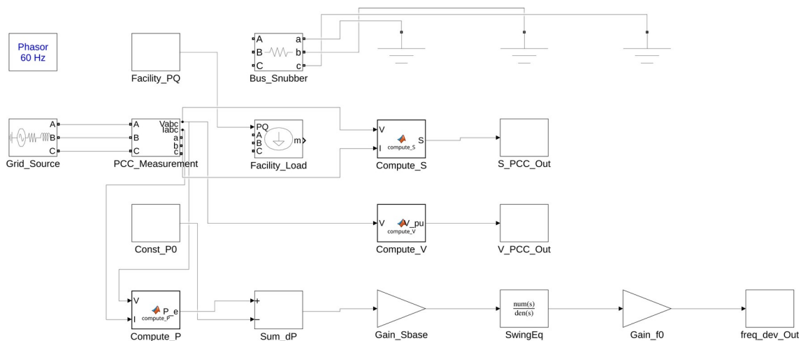
Figure 7. Simulink Block for Grid
