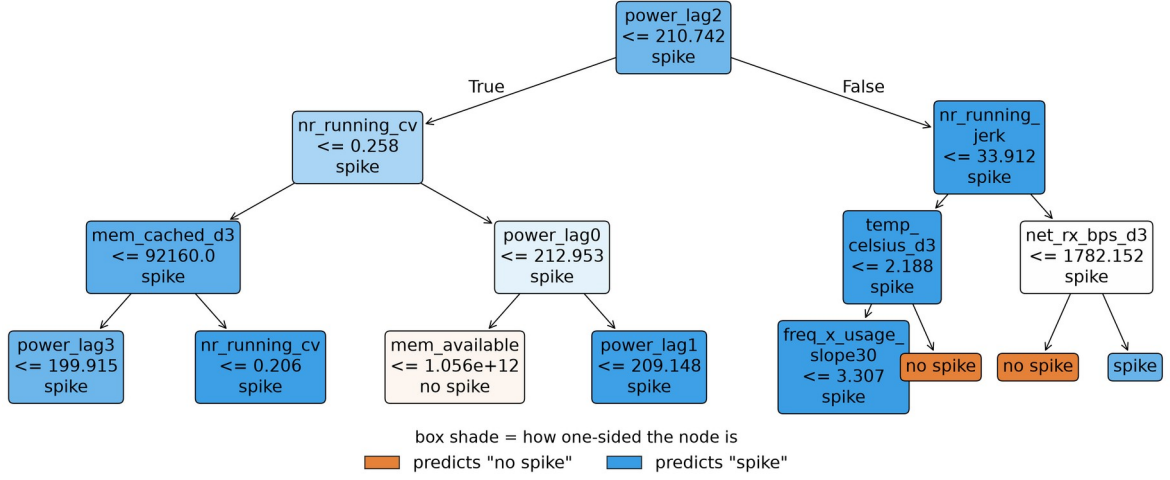
Figure 6. RF Detector Example Decision Tree
