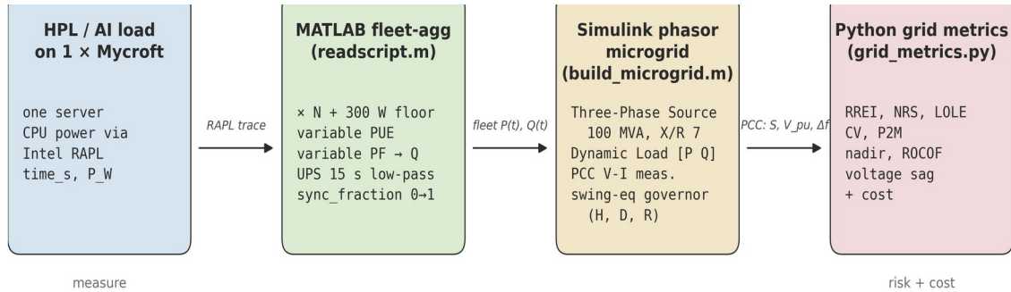
Figure 8. Mycroft to Grid Simulation Pipeline
