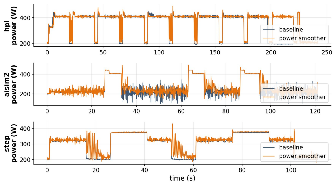
Figure 18. Ramp Down (Power Smoother) vs workloads
