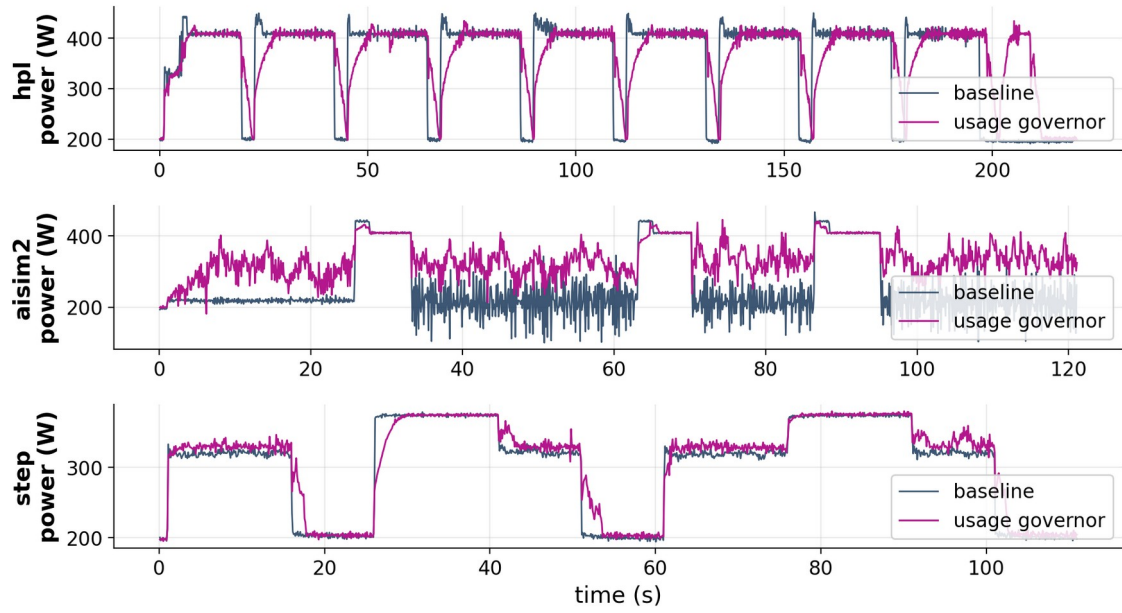
Figure 19. Governor (usagegov) vs workloads
