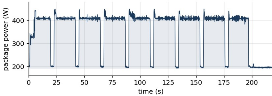
Figure 14. ai_load.sh (HPL)
