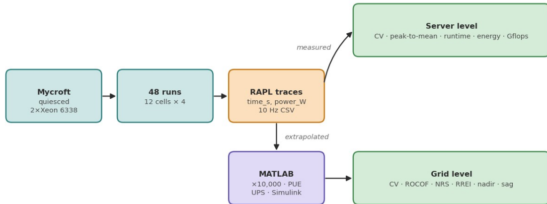
Figure 13. Analysis Pipeline
