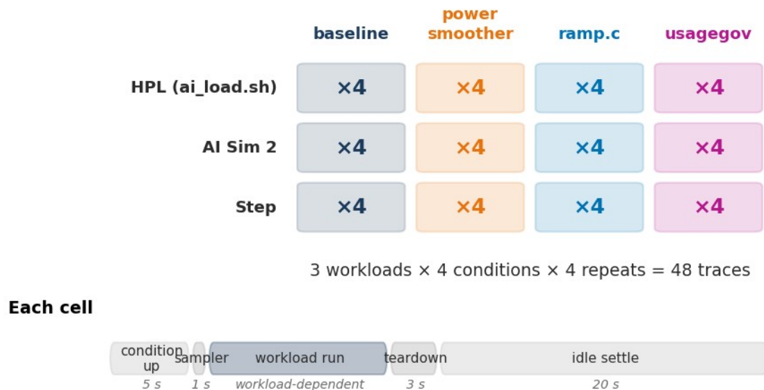
Figure 12. Run Matrix
