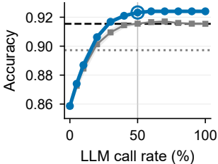
(a) CLEF 2024
