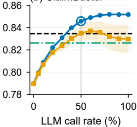
(b) ClaimBuster
