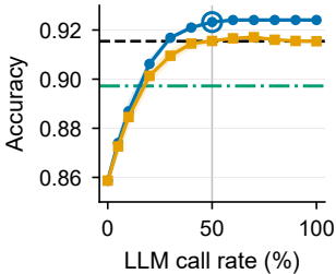
(a) CLEF 2024
