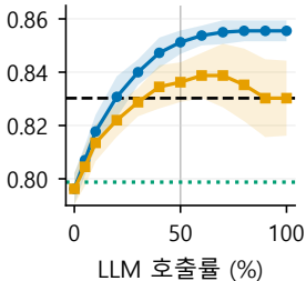
(b) ClaimBuster (n=800)
