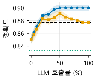
(a) CLEF 2024 (n=318)
