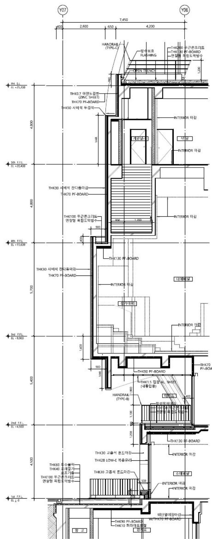
2 Exterior Wall Detail - 18 SCALE : 1/200
