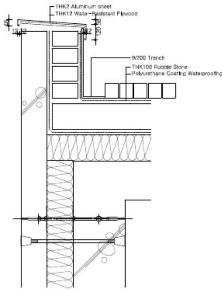
B. Parapet in Thermomass Concrete System
