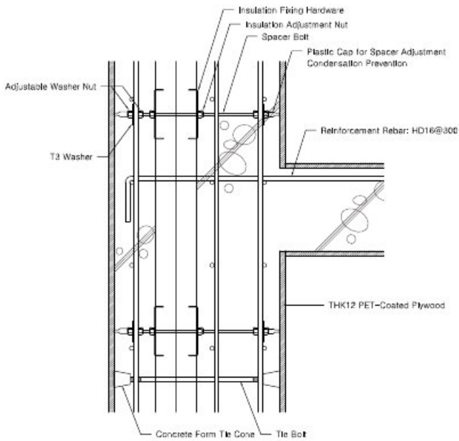
C. Thermomass Concrete System
