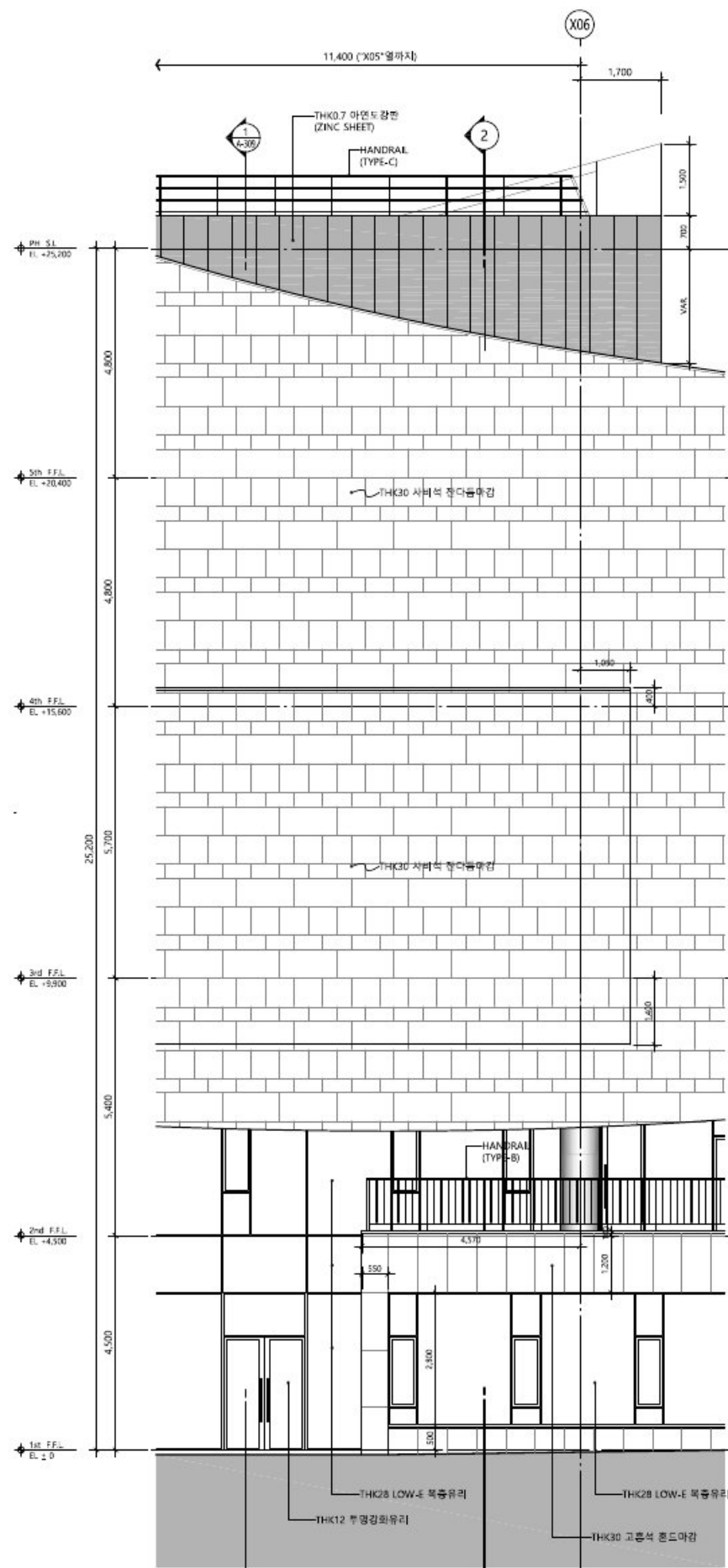
1 Exterior Wall Detail - 17 SCALE : 1/200
