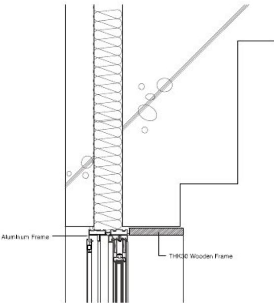
D. Window Installation
