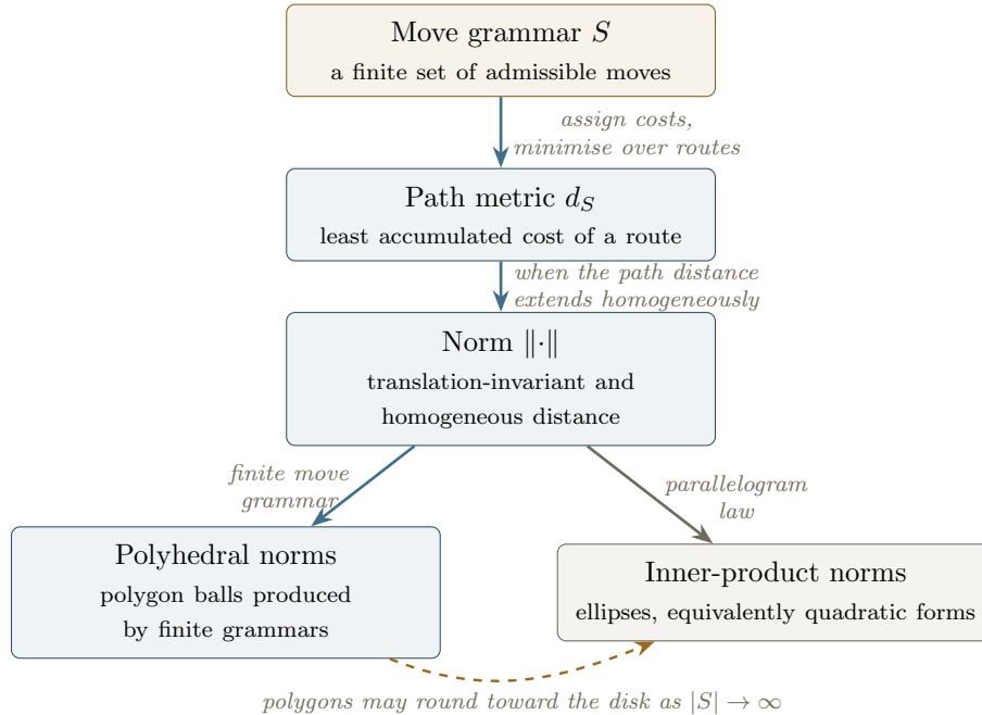
Figure 2: The family generated from a move grammar. A finite set of admissible moves with positive costs first gives a path metric by least-cost routing. In favourable lattice cases this path metric is the restriction of a norm. From the norm node the diagram branches: finite grammars give polyhedral norms, while inner-product norms are selected by the parallelogram law and have ellipses as unit balls. The Euclidean disk is therefore a limiting ideal for finite move grammars rather than another finite grammar.
