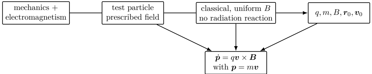
Figure 3: Charged-particle model is produced by successive choices, not by the Lorentz equation alone.
