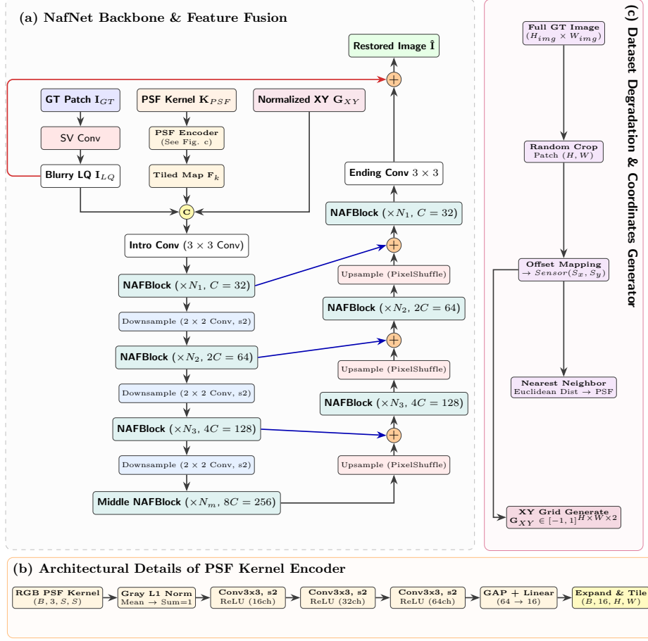
Figure 1: Overview of the proposed PSF-guided NafNet framework. (a) The primary NafNet U-Net backbone receiving concatenated Blurry LQ Image, PSF feature maps, and Normalized XY Spatial Coordinates. (b) Architectural details of the PSFKernelEncoder and tiling mechanism. (c) The online dataset degradation processing pipeline deriving local PSF kernels and normalized sensor grids.
