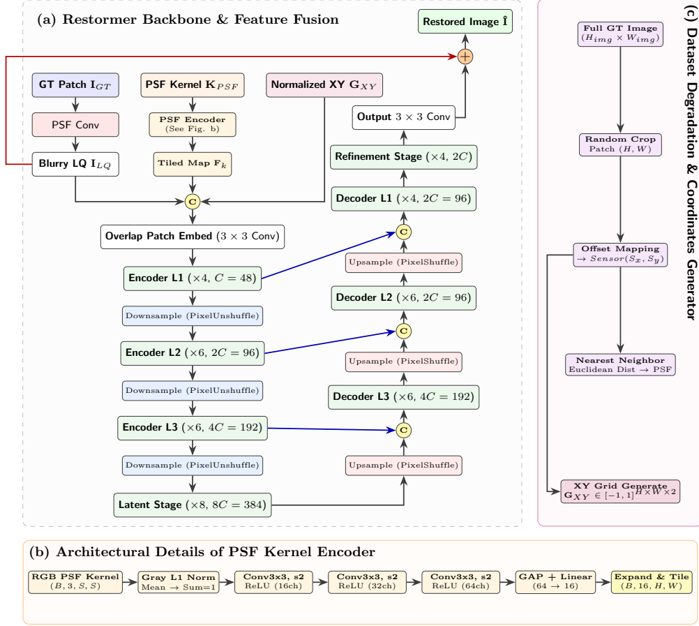
Figure 1: Overview of the proposed PSF-guided Restormer framework. (a) The primary Restormer U-Net backbone receiving concatenated Blurry LQ Image, PSF feature maps, and Normalized XY Spatial Coordinates. (b) Architectural details of the PSFKernelEncoder and tiling mechanism. (c) The online dataset degradation processing pipeline deriving local PSF kernels and normalized sensor grids.
