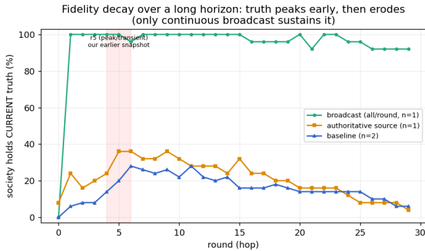
Figure 2: Long-horizon fidelity decay. Held current-truth rises early (peak near round 6) then erodes toward a low steady state; an authoritative source decays too, converging to baseline, while only continuous broadcast sustains truth. A short-horizon snapshot at round 5 therefore slightly overstates long-run retention.
