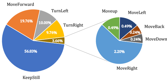
Figure 12: The proportion of different actions taken by Collector.
