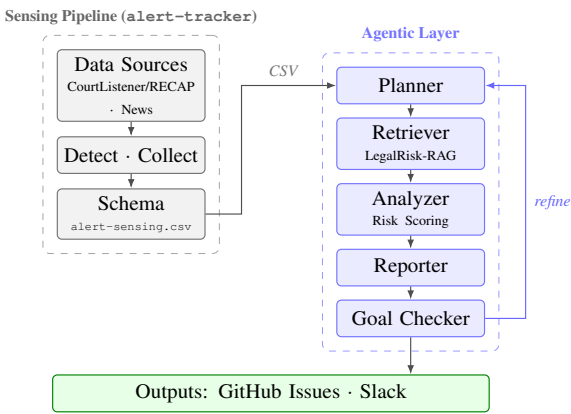
Figure A.1: ALERT architecture. The sensing pipeline (left) detects filings, collects documents, and populates the schema; the agentic layer (right) plans, retrieves time-valid precedent, scores risk, and reports, with the Goal Checker driving a refine loop until evidence coverage is met.
