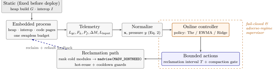
Figure 1: SAGE-MM runtime composition and the narrow online action space (reclamation interval T and compaction gate). Static interventions (heap build G , interop I ) sit upstream and reduce the pressure presented to the controller; only the control path adapts online. Per-interval telemetry is normalized into a dimensionless pressure, the interchangeable policy emits the two bounded actions, and the reclamation path issues madvise (MADV_DONTNEED) through the conservative native helper under the hot-reuse and cooldown guards. The dashed band marks the policy-independent fail-closed and adverse-regime supervisory guards.
